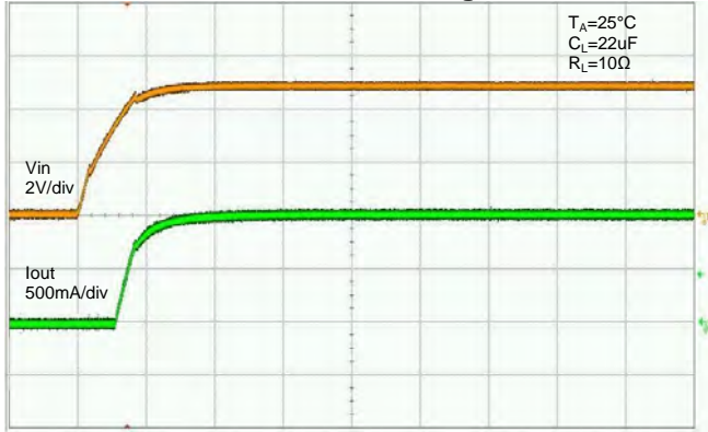
UVLO Increasing
