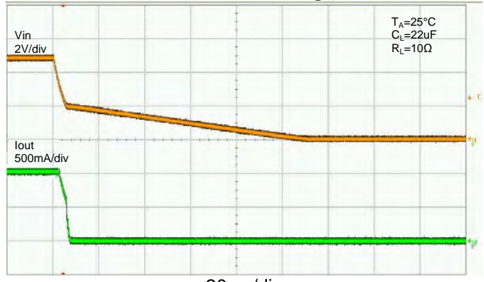
UVLO Decreasing
