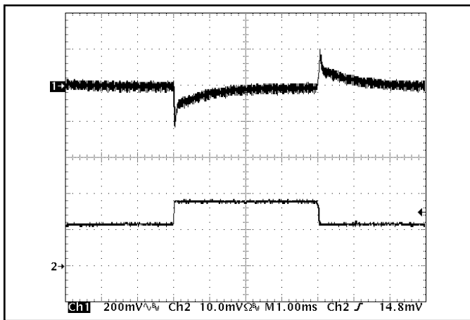
Figure 11: Output voltage response to step-change in load current (50%-75%-50% of I out (max); dI/dt = 0.1A/μs). Load cap: 15μF, 100 mΩ ESR tantalum cap and 1μF ceramic cap. Ch 1: V out (200mV/div), Ch 2: I out (2A/div).
