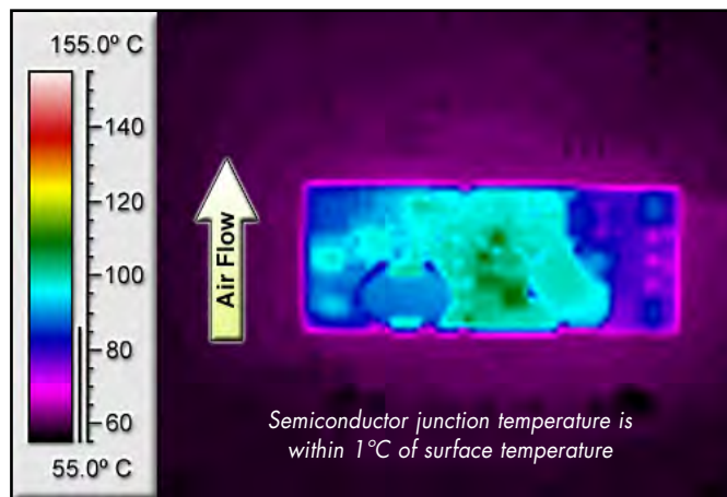
Figure 6: Thermal plot of converter at 5 amp load current (75W) with 55°C air flowing at the rate of 200 LFM. Air is flowing across the converter from pin 3 to pin 1 (nominal input voltage).
