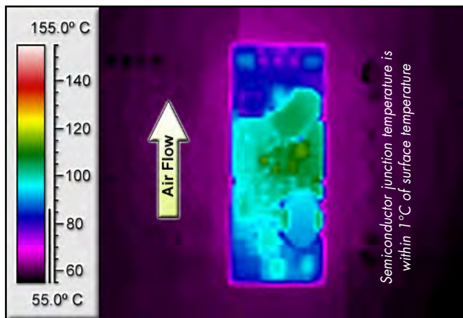
Figure 8: Thermal plot of converter at 5 amp load current (75W) with 55°C air flowing at the rate of 200 LFM. Air is flowing across the converter from input to output (nominal input voltage).
