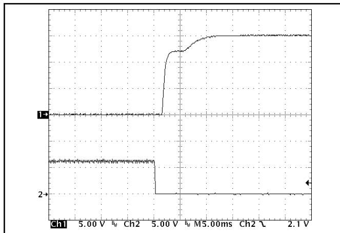
Figure 10: Turn-on transient at zero load (5 ms/div). Ch 1: V out (5V/div). Ch 2: ON/OFF input (5V/div).
