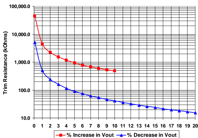
Figure C: Trim Graph
