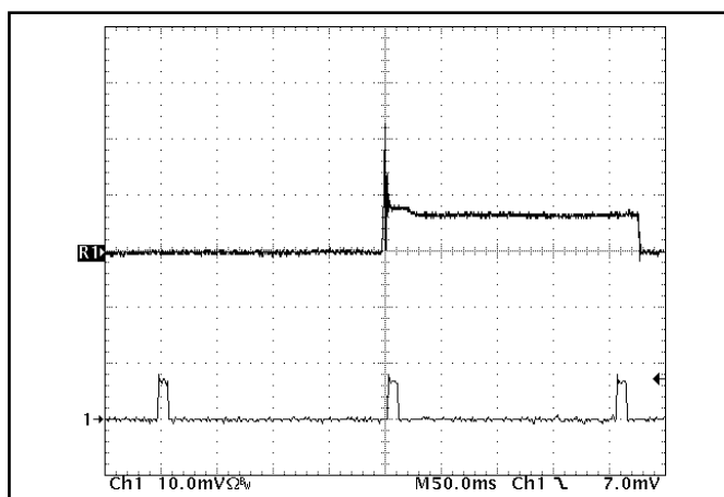
Figure 18: Load current ( 10\ \text{A}/\text{div} ) as a function of time when the converter attempts to turn on into a 1\ \text{m}\Omega short circuit. Top trace ( 2\text{ms}/\text{div} ) is an expansion of the on-time portion of the bottom trace.
