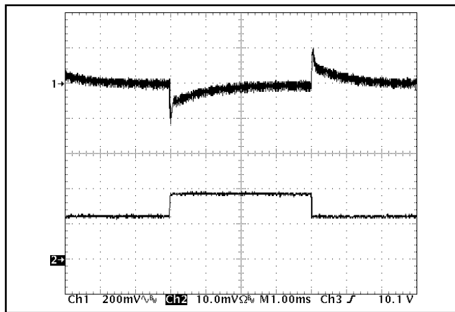
Figure 12: Output voltage response to step-change in load current (50%-75%-50% of I out (max); dI/dt = 0.5A/μs). Load cap: 470μF, 15μF, 100 mΩ ESR tantalum cap and 1μF ceramic cap. Ch 1: V out (200mV/div), Ch 2: I out (2A/div).
