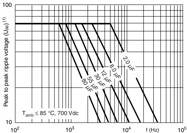
(1) Limited by maximum ripple voltage 0.1 \times U_{Ndc}
