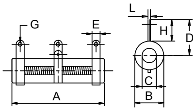
Power Adjustable Resistor (DRS-A) N - No mount Dimensions
