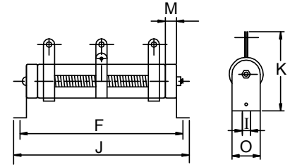
Power Adjustable Resistor (DRS-A) G - Horizontal mount Dimensions
