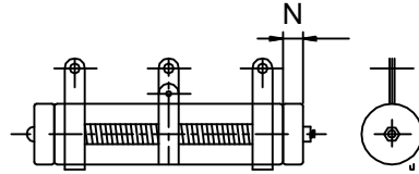
Power Adjustable Resistor (DRS-A) Z - Vertical mount Dimensions
