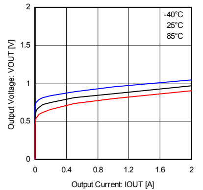
Fig.24 Low side body diode (2A class)
