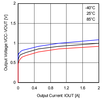
Fig.18 High side body diode (2A class)
