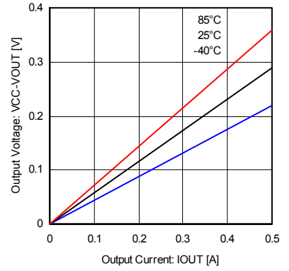
Fig.15 Output high voltage (2A class)
