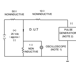
FIG.6-TEST CIRCUIT DIAGRAM AND REVERSE RECOVERY TIME CHARACTERISTIC
