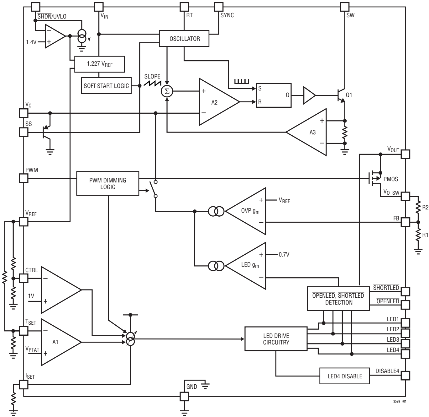
Figure 1. Block Diagram
