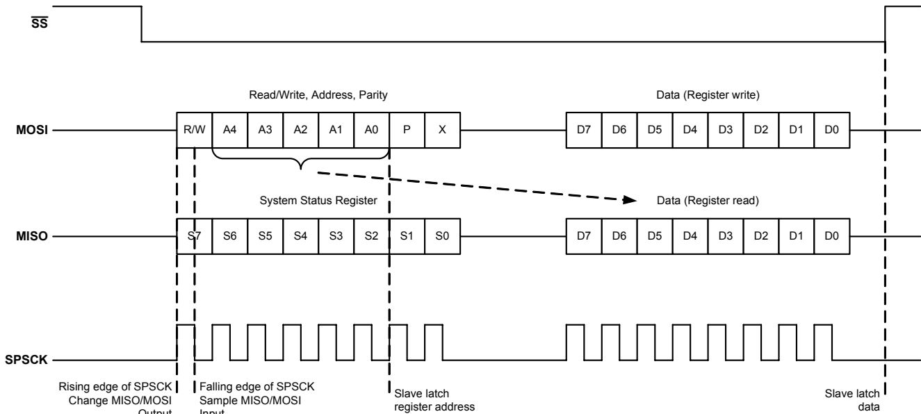
Figure 11. SPI Protocol
