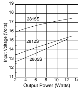
MHF Single Low Line Dropout
