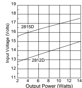
MHF Dual Low Line Dropout
