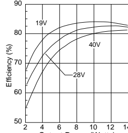
MHF2815D Efficiency
