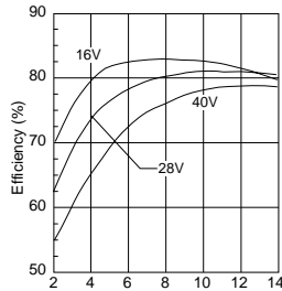
MHF2812D Efficiency
