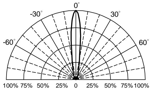
Fig.6 Directivity Radiation
