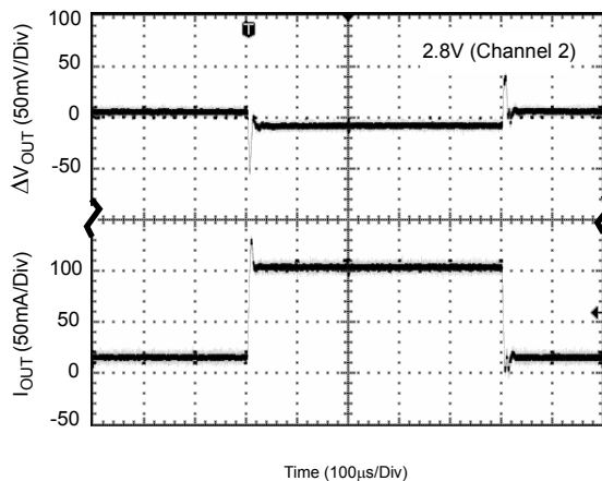
Figure 39. Load Transient
