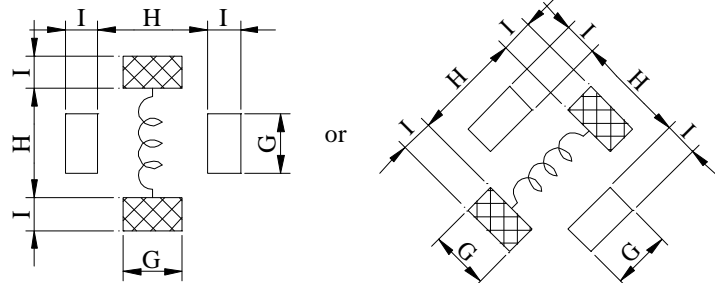
( PCB Pattern )
