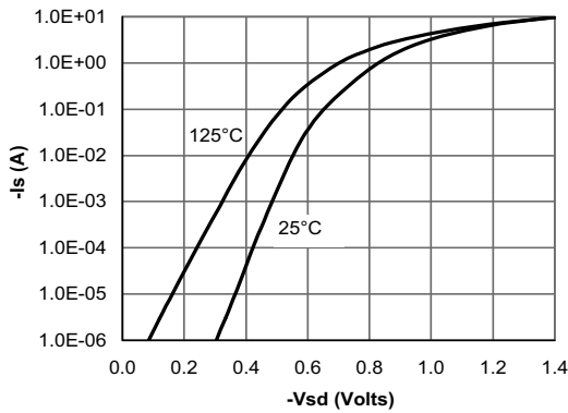
Figure 6: Body-Diode Characteristics
