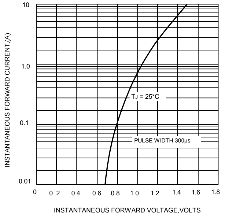
FIG.4-TYPICAL FORWARD CHARACTERISTICS
