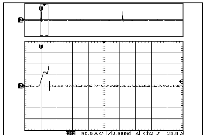
Figure 18: Load current (50A/div) as a function of time when the converter attempts to turn on into a 1\ \text{m}\Omega short circuit. Bottom trace (2ms/div) is an expansion of the on-time portion of the top trace.
