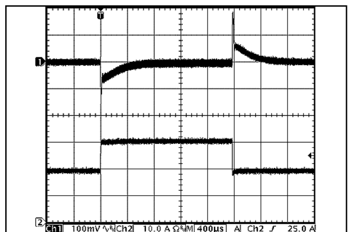
Figure 12: Output voltage response to step-change in load current (50%-75%-50% of I_{out(max)} ; dI/dt = 1A/\mu s ). Load cap: 470 \mu F , 30 m \Omega ESR tantalum capacitor and 1 \mu F ceramic cap. Ch 1: V_{out} (100mV/div), Ch 2: I_{out} (10A/div).
