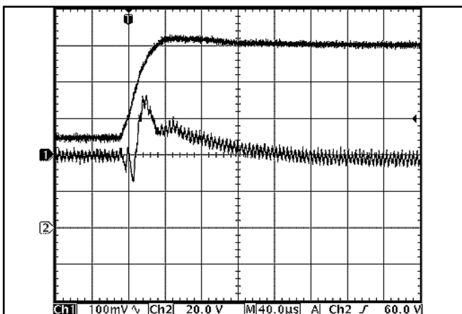
Figure 17: Output voltage response to step-change in input voltage (50V to 100V in 40 \mu\text{s} ). Load cap: 10\ \mu\text{F} , 100\ \text{m}\Omega ESR tantalum capacitor and 1\ \mu\text{F} ceramic cap. Ch 1: V_{out} (100mV/div), Ch 2: V_{in} (20V/div).
