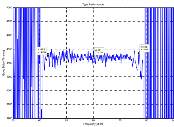
Group Delay Variation(f0±8.5MHz)
