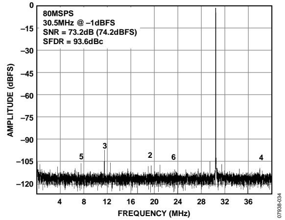
Figure 9. AD9251-80 Single-Tone FFT with f_{IN} = 30.5 MHz
