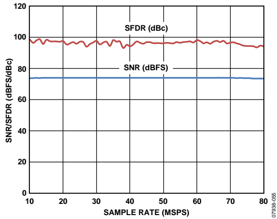
Figure 13. AD9251-80 SNR/SFDR vs. Sample Rate with f_{IN} = 9.7 MHz
