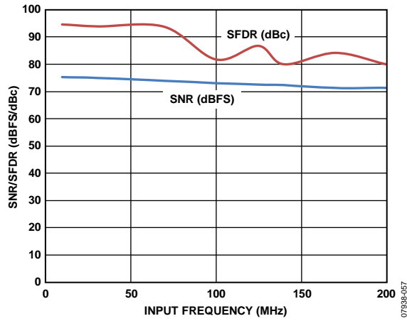
Figure 12. AD9251-80 SNR/SFDR vs. Input Frequency (AIN) with 2 V p-p Scale
