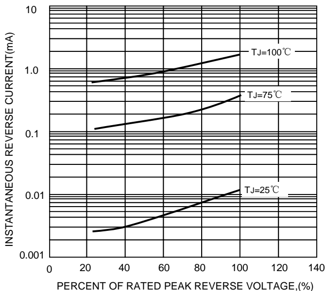
FIG.2-TYPICAL REVER CHARACTERISTICS
