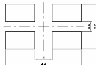
Recommended Soldering Pad Layout
