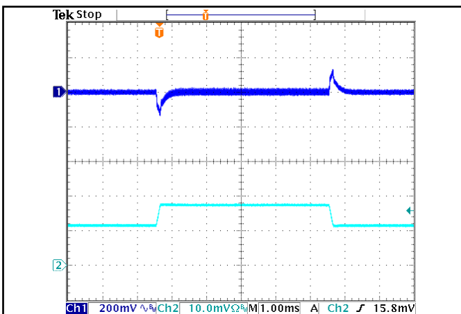
Figure 5: Output voltage response to step-change in load current (50%-75%-50% of I out (max)); di/dt = 0.1 \text{ A}/\mu\text{s} . Load cap: 15 \mu\text{F} Tantalum + 1 \mu\text{F} Ceramic capacitor. Ch 1: V out (200 mV/div), Ch 2: I out (20 A/div).
