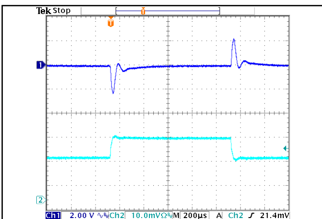
Figure 5: Output voltage response to step-change in load current (50%-75%-50% of I out (max); dl/dt = 0.1 A/μs). Load cap: 1 μF ceramic capacitor. Ch 1: Vout (2 V/div), Ch 2: Iout (2 A/div).
