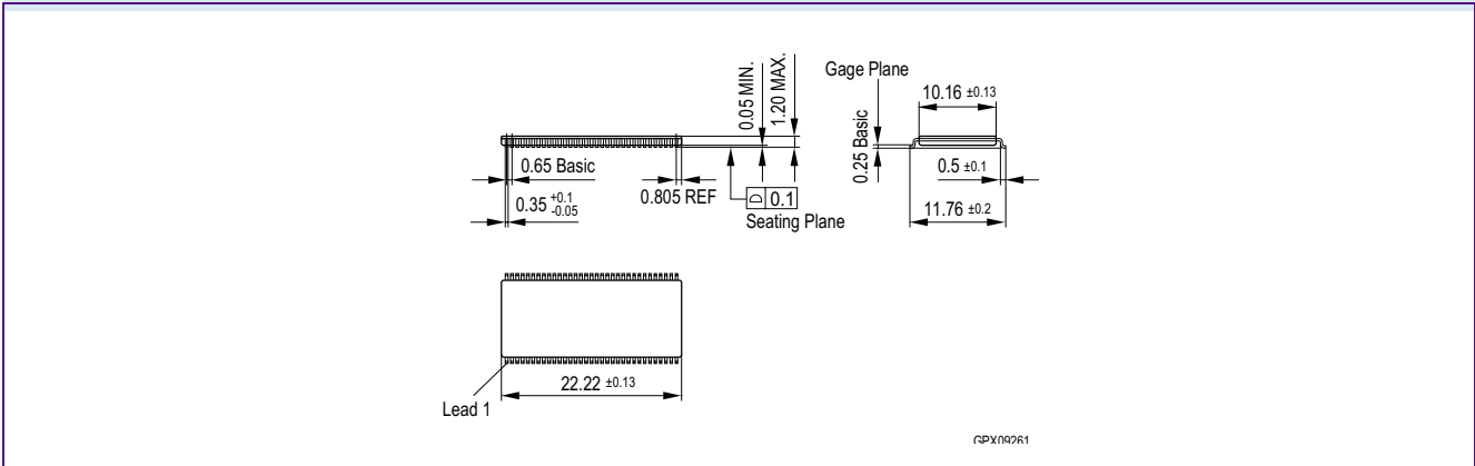
FIGURE 5 Package Outline of P-TSOPII-66-1-1 (green/non-green)
