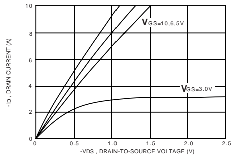
Figure 1. Output Characteristics
