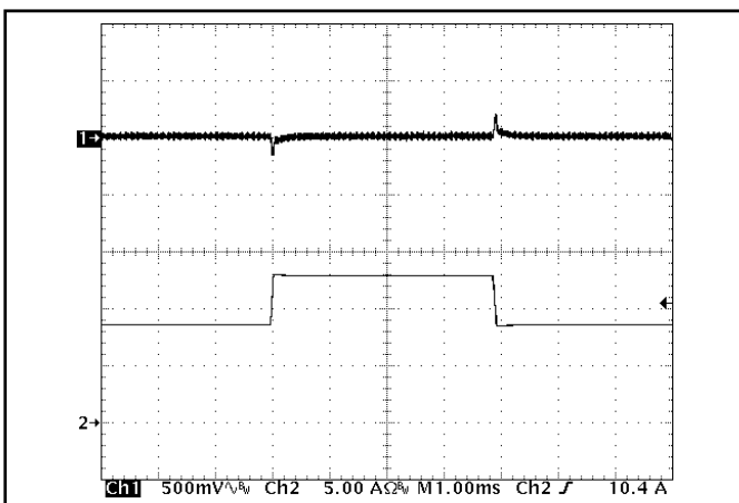
Figure 5: Output voltage response to step-change in load current (50%-75%-50% of I out (max); dl/dt = 0.1 A/us). Load cap: 1 μF ceramic and 15 μF tantalum capacitors. Ch 1: V out (500 mV/div), Ch 2: I out (5 A/div).
