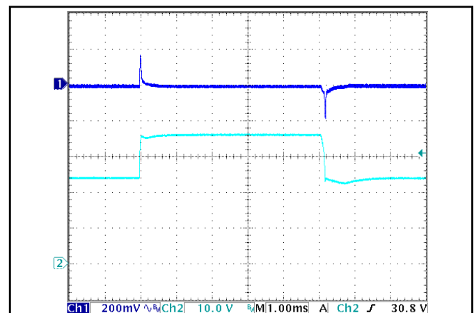
Figure 6: Output voltage response to step-change in input voltage (250 V/ms). Load cap: 100 μF, electrolytic output capacitance. Ch 1: V out (200 mV/div), Ch 2: V in (10 V/div).
