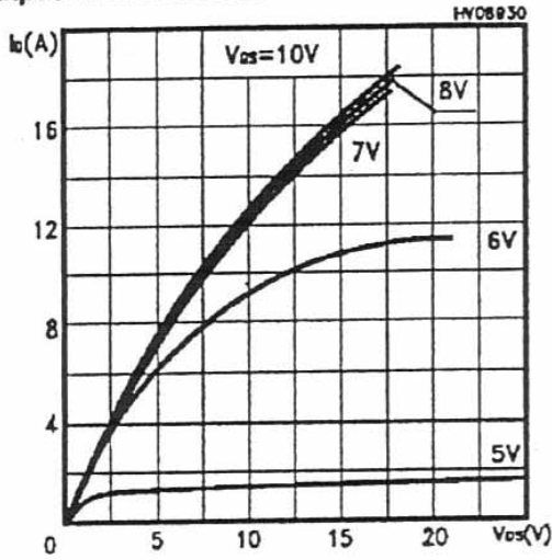
Output Characteristics
