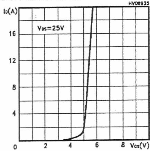
Transfer Characteristics
