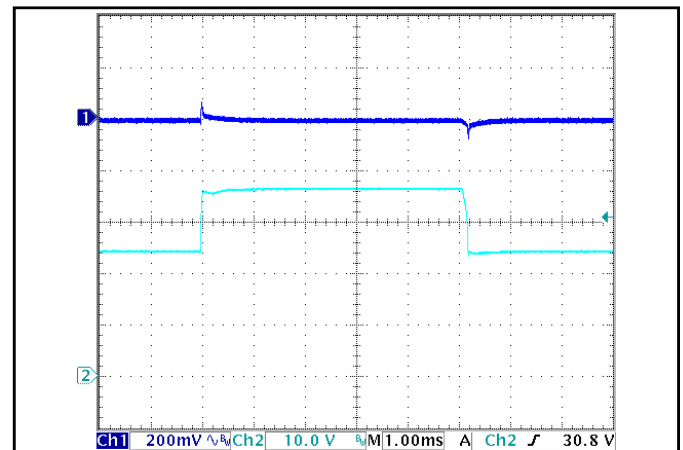
Figure 6: Output voltage response to step-change in input voltage (250 V/ms). Load cap: 100 \mu\text{F} , electrolytic output capacitance. Ch 1: V out (200 mV/div), Ch 2: V in (10 V/div).
