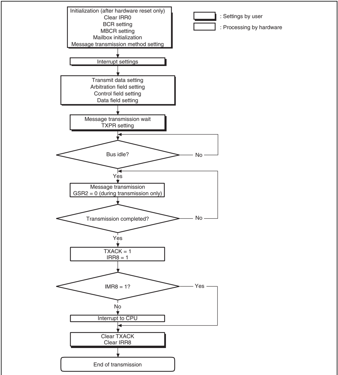
Figure 18.9 Transmission Flowchart
