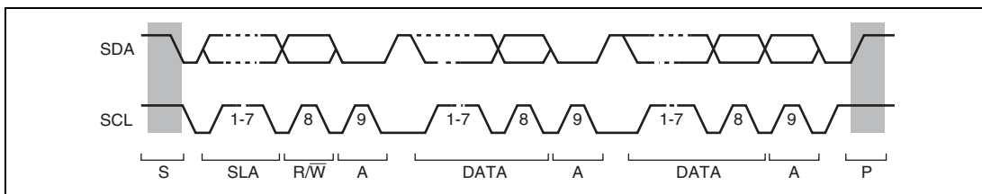
Figure 14.4 I 2 C Bus Timing
