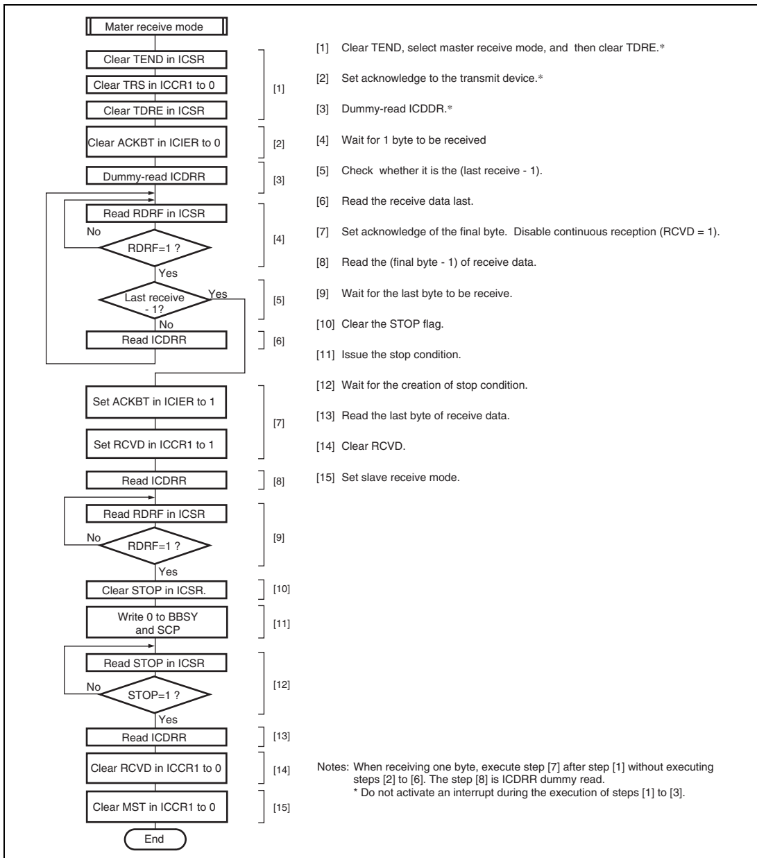
Figure 14.18 Sample Flowchart for Master Receive Mode
