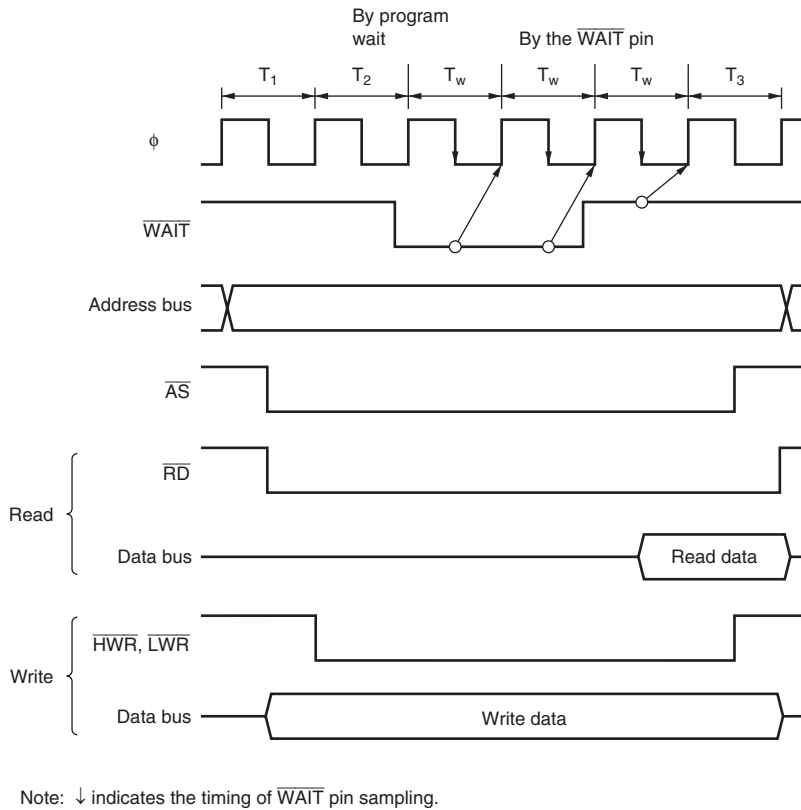
Figure 7.24 Example of Wait State Insertion Timing
