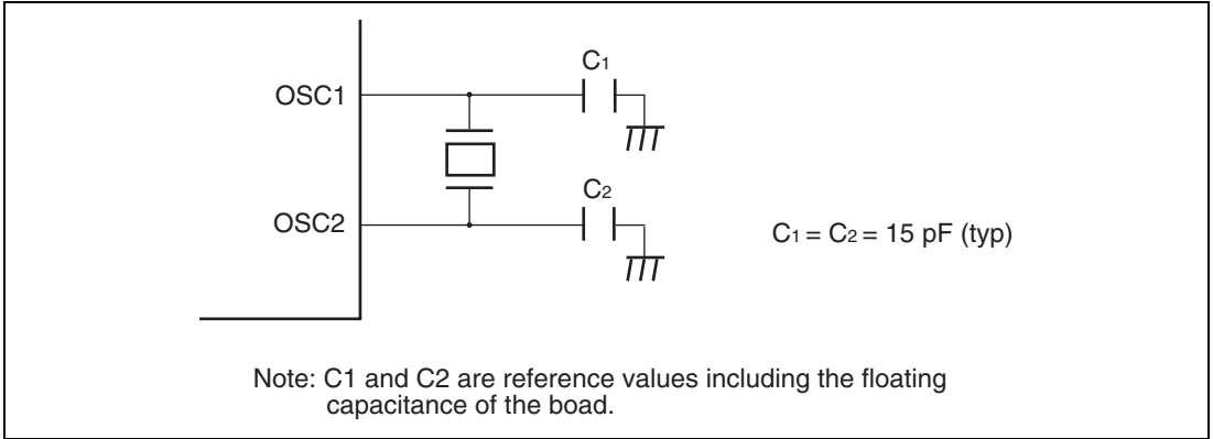
Figure 21.8 Connection Example of 32.768-kHz Crystal Resonator
