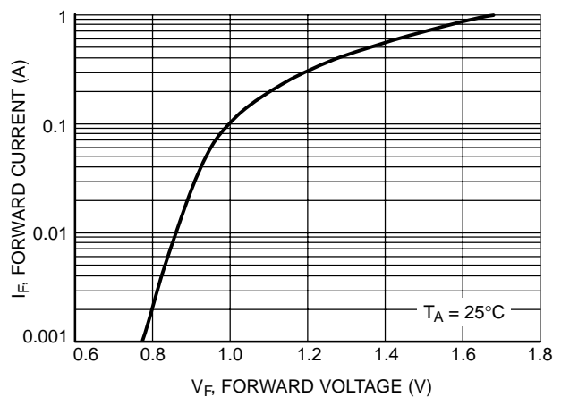
Figure 6. Forward Voltage
