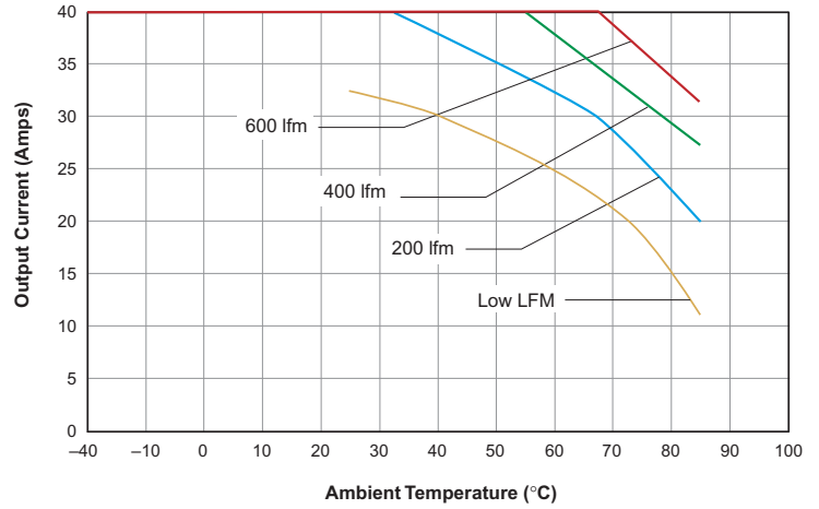
USQ-1.5/40-D48: Output Current vs. Ambient Temperature (Transverse air flow, pin 1 to pin 3; V IN = 48V, no heat sink.)
