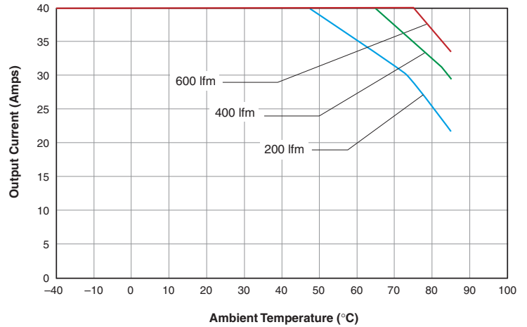
USQ-1.5/40-D48: Output Current vs. Ambient Temperature (Longitudinal air flow, pin 1 to pin 3; V IN = 48V, 1/2" heat sink.)
