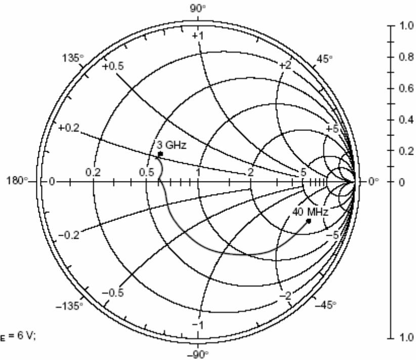
Common emitter input reflection coefficient ( S_{11} )
