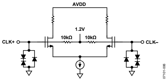
Figure 15. Clock Inputs
