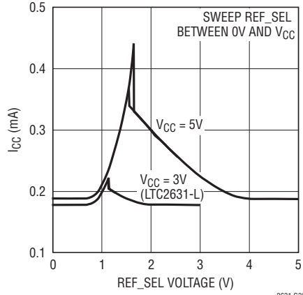
Supply Current vs REF_SEL Voltage
