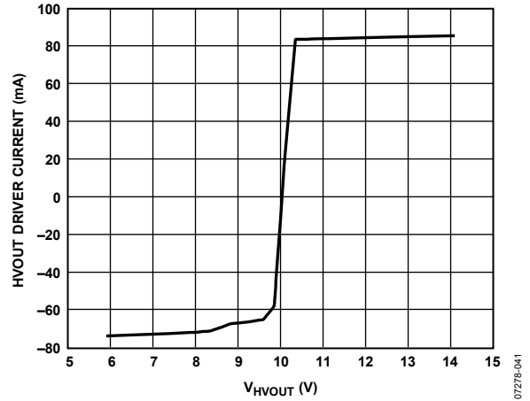
Figure 32. HVOUT VHH Current Limit; V_{HH} = 10.0 V; V_{HVOUT} Swept from 5.9 V to 14.1 V
