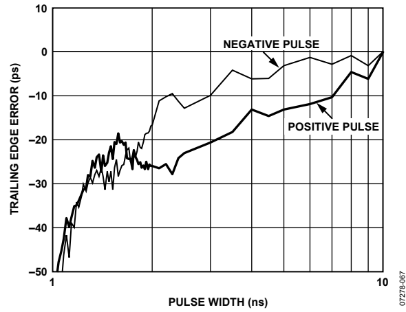
Figure 18. Driver Minimum Pulse Width; V_H = 3.0\text{ V} ; V_L = 0.0\text{ V}
