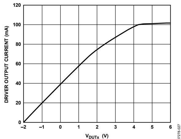
Figure 26. Driver Output Current Limit; Driver Programmed to -2.0 V; V DUTx Swept from -2.0 V to +6.0 V
