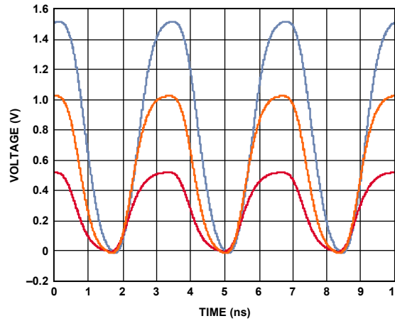
Figure 7. 300 MHz Driver Response; V_H = 1.0\text{ V}, 2.0\text{ V}, 3.0\text{ V}; V_L = 0.0\text{ V}; 50\ \Omega Termination
