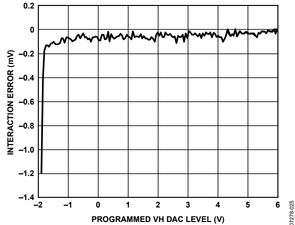
Figure 24. Driver Interaction Error; VL = -2.0 V; VH Swept from -1.9 V to +6.0 V
