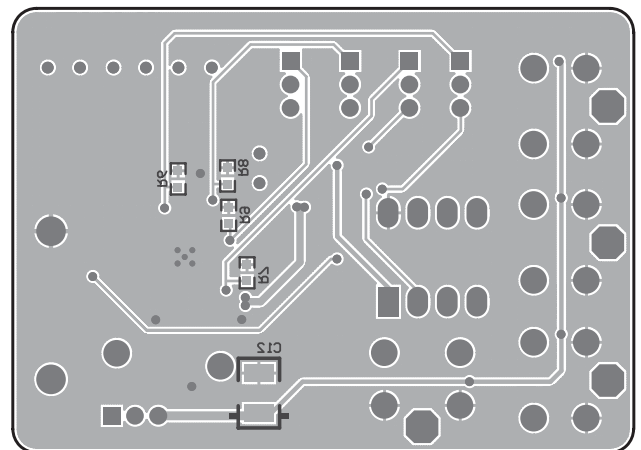
Figure 7: AAT2846 Evaluation Board Layout Bottom Side.
