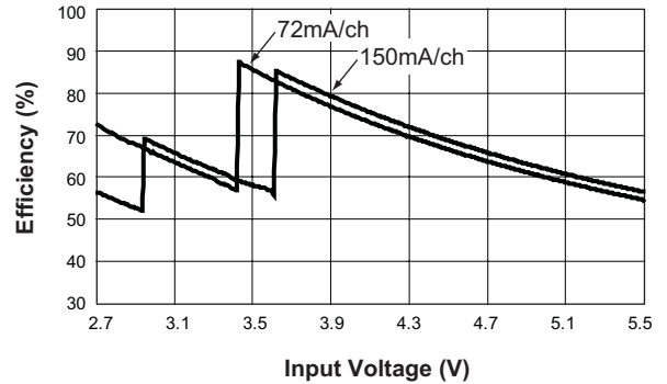
Flash Efficiency vs. Input Voltage
