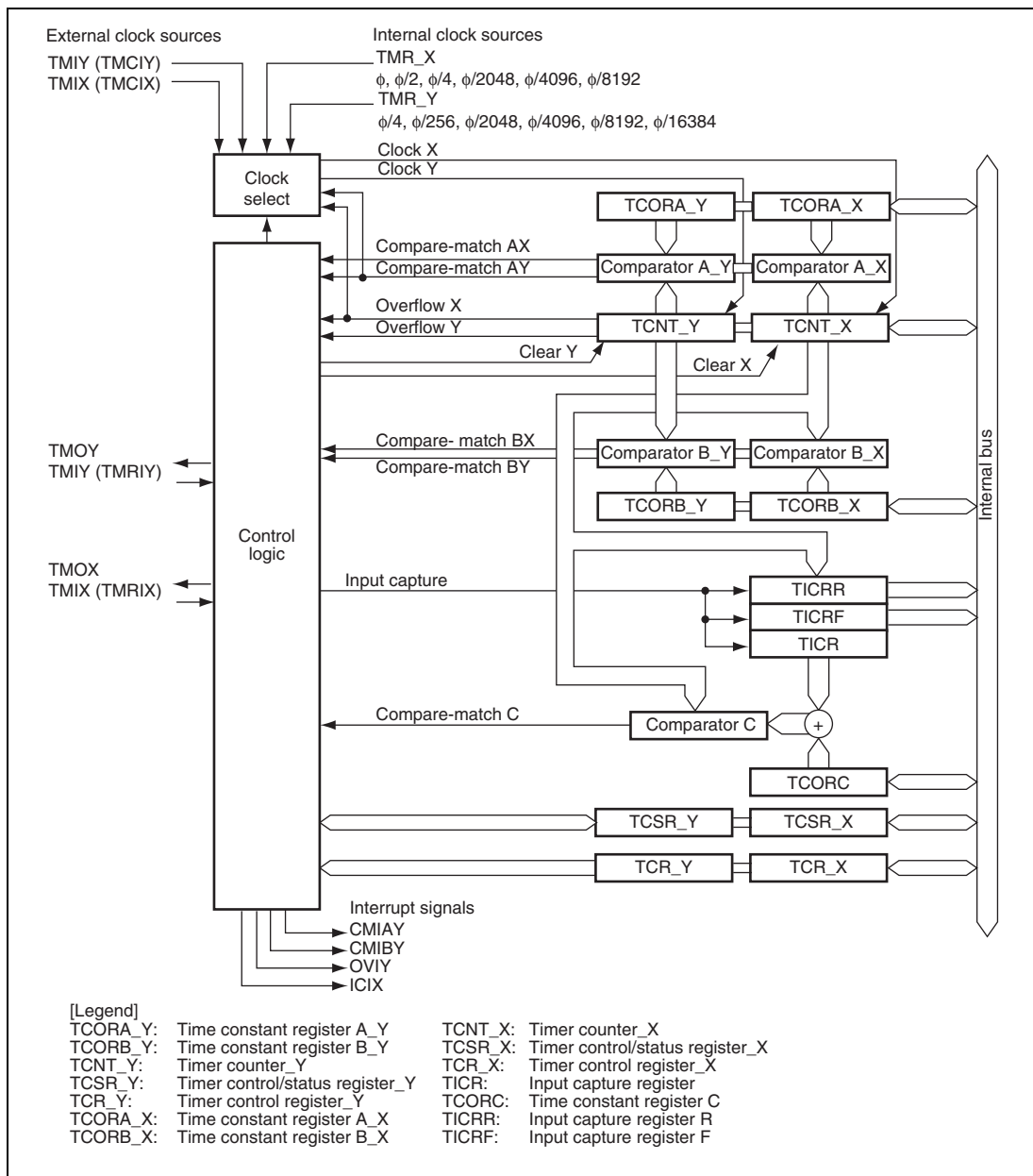
Figure 11.2 Block Diagram of 8-Bit Timer (TMR_Y and TMR_X)
