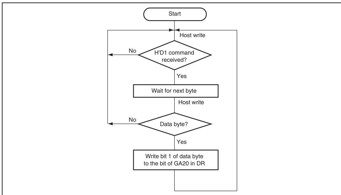
Figure 16.4 GA20 Output
