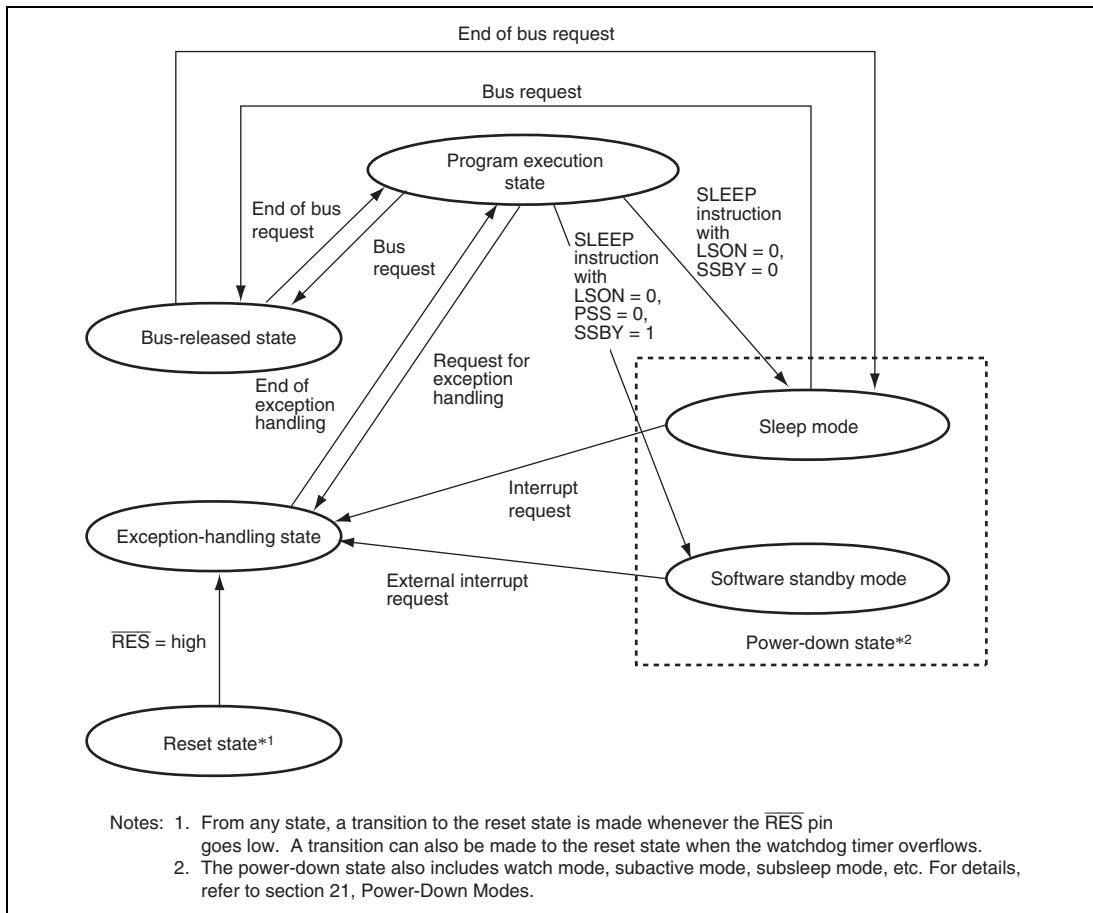
Figure 2.13 State Transitions
