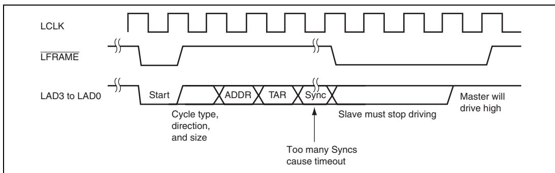
Figure 16.3 Abort Mechanism
