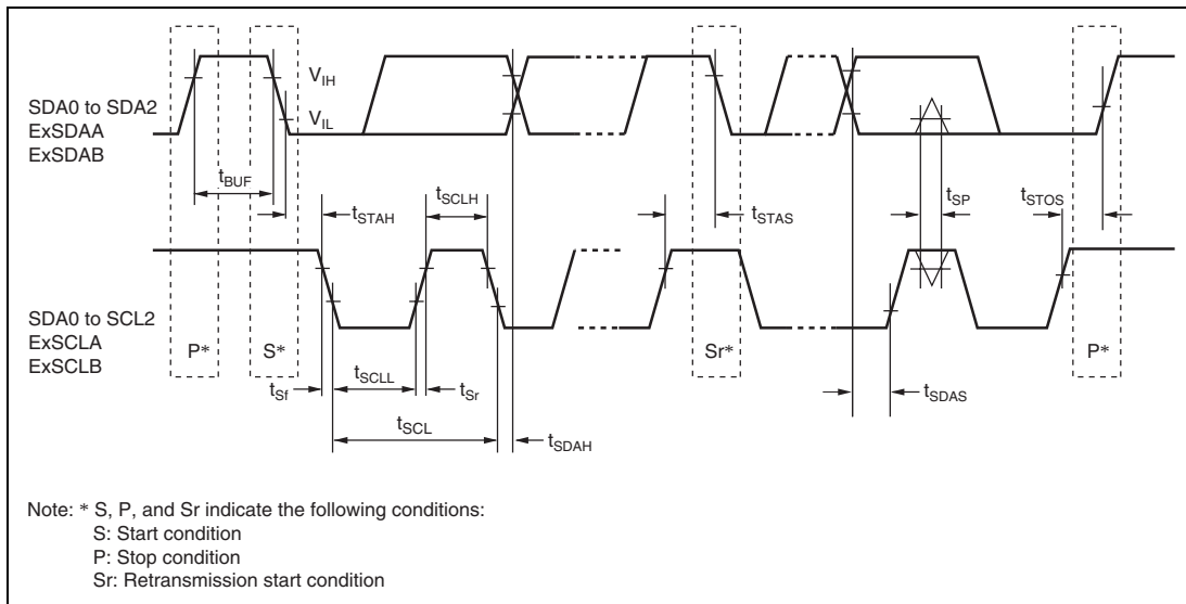
Figure 23.19 I²C Bus Interface Input/Output Timing
