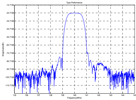
Frequency Respond
