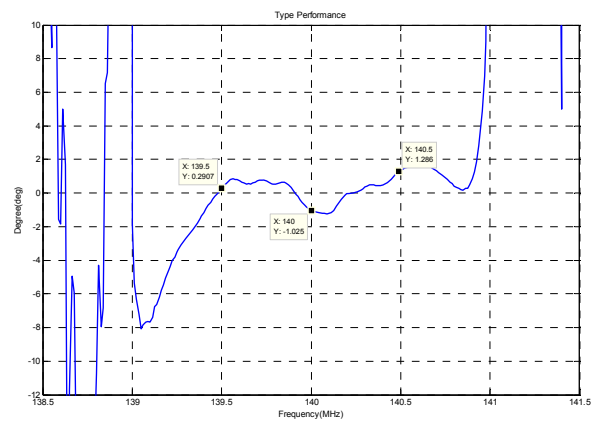
Phase Linearity(f0±0.5MHz)
