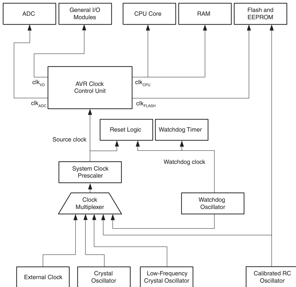
Figure 6-1. Clock Distribution
