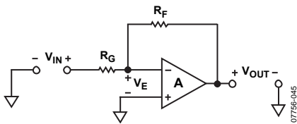
Figure 39. Inverting Configuration
