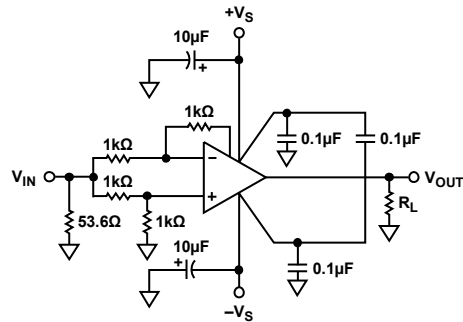
Figure 37. Common-Mode Rejection
