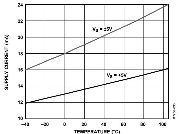
Figure 29. Quiescent Current vs. Temperature for Various Supply Voltages
