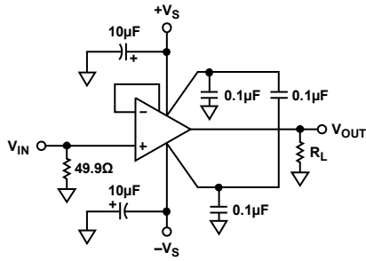
Figure 32. G = 1 Configuration
