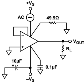
Figure 33. Positive Power Supply Rejection
