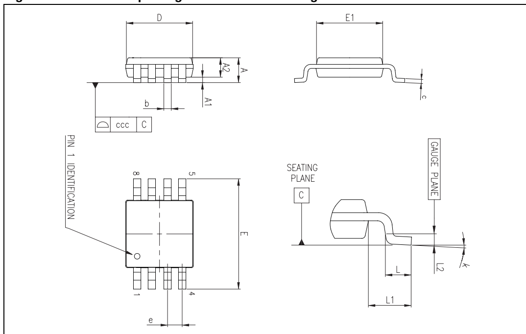
Figure 15. MiniSO-8 package mechanical drawing
