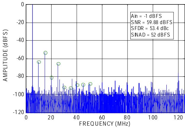
FIGURE 20. SINGLE-TONE SPECTRUM @ 495MHz
