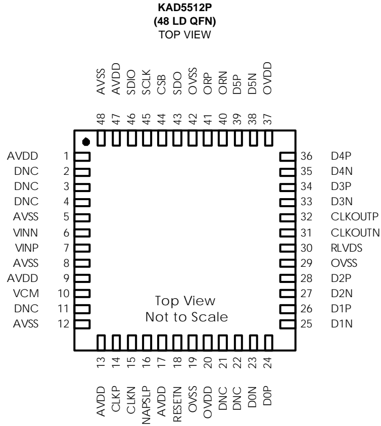
FIGURE 4. PIN CONFIGURATION
