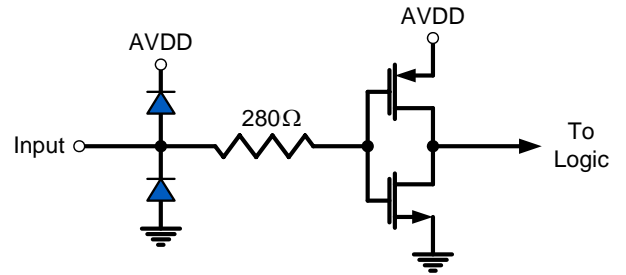
FIGURE 46. DIGITAL INPUTS
