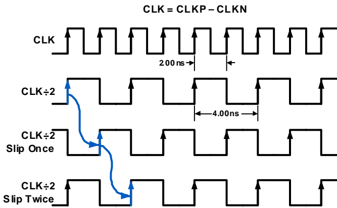
FIGURE 40. PHASE SLIP: CLK÷2 MODE, f CLK = 500MHz
