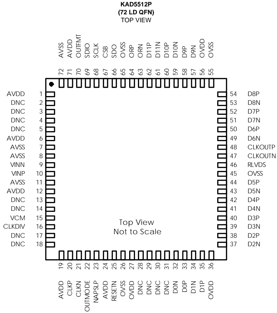
FIGURE 3. PIN CONFIGURATION
