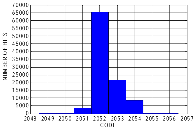
FIGURE 15. NOISE HISTOGRAM
