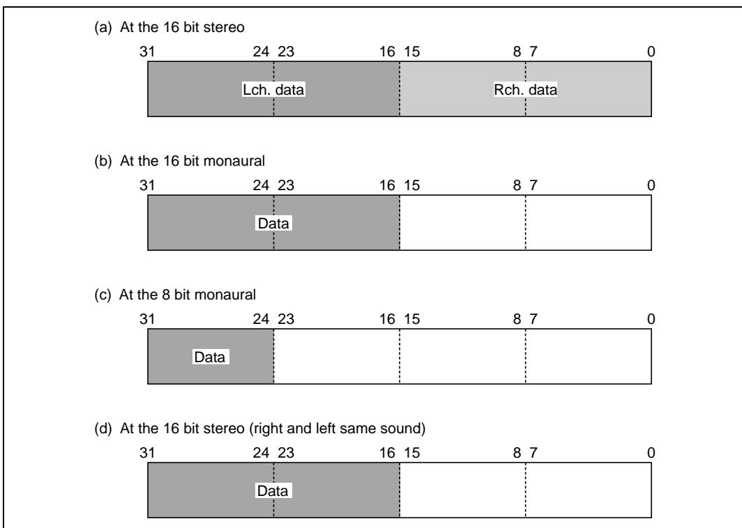
Figure 20.5 Transmit or Receive Data Bit Alignment
