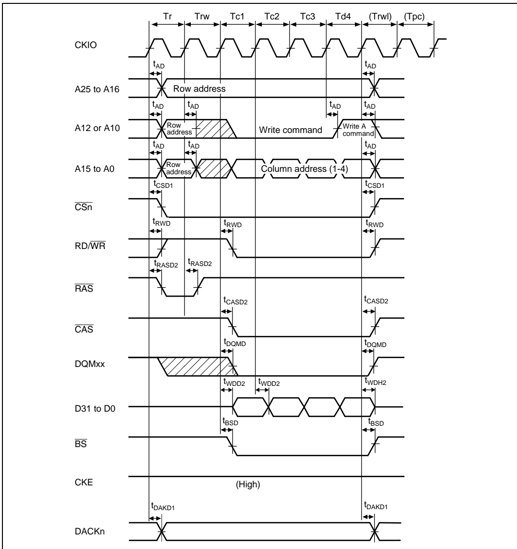
Figure 32.30 Synchronous DRAM Write Bus Cycle (Burst Mode (Single Write x 4), RCD = 1, TPC = 0, TRWL = 0)
