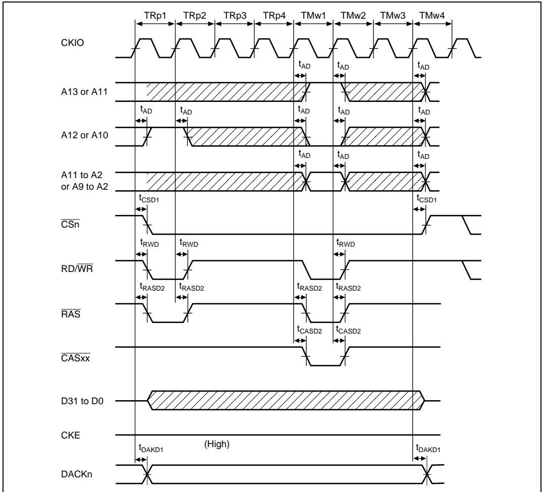
Figure 32.33 Synchronous DRAM Mode Register Write Cycle
