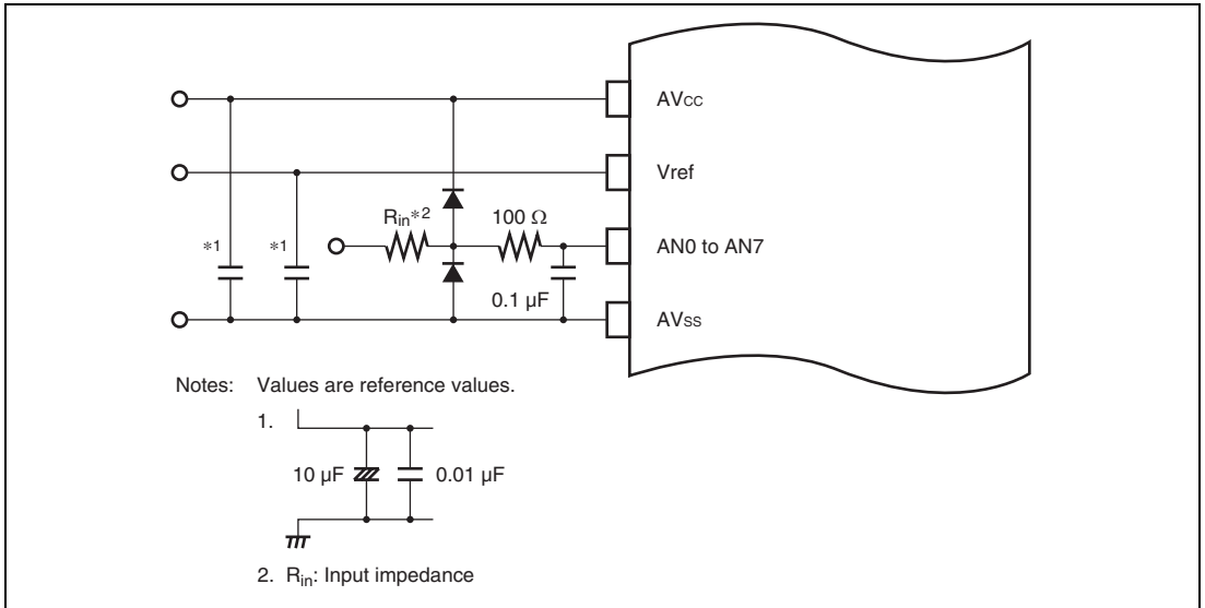
Figure 19.13 Example of Analog Input Protection Circuit
