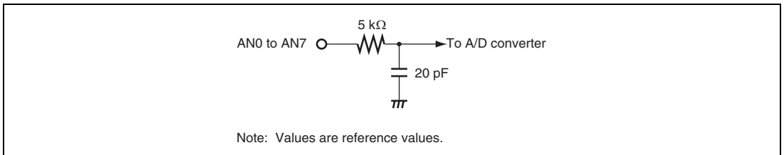
Figure 19.14 Analog Input Pin Equivalent Circuit
