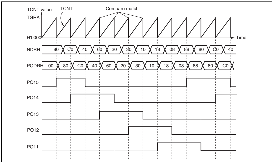
Figure 14.7 Normal Pulse Output Example (5-Phase Pulse Output)
