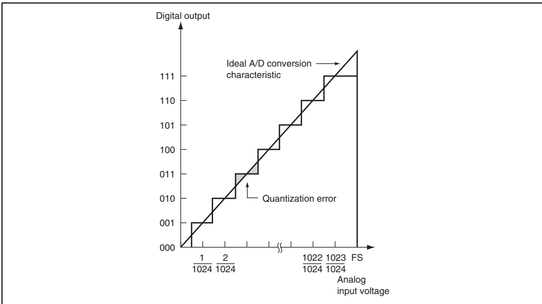
Figure 19.9 A/D Conversion Accuracy Definitions
