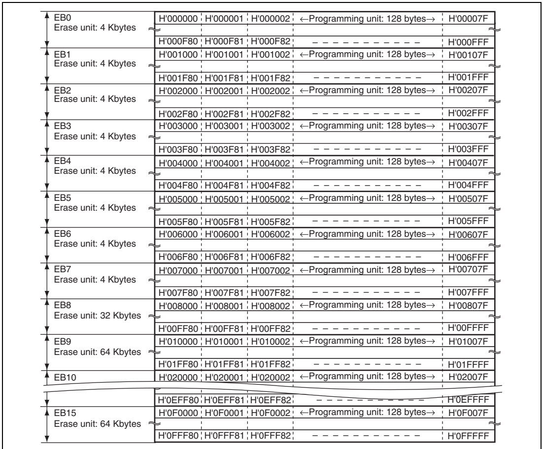
Figure 22.4 (2) User MAT Block Structure of H8SX/1634
