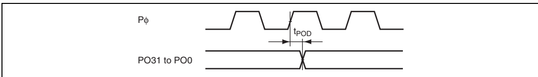
Figure 27.28 PPG Output Timing
