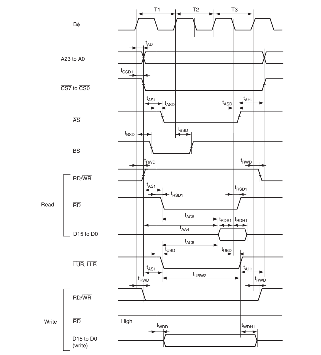
Figure 27.14 Byte Control SRAM: Three-State Read/Write Access
