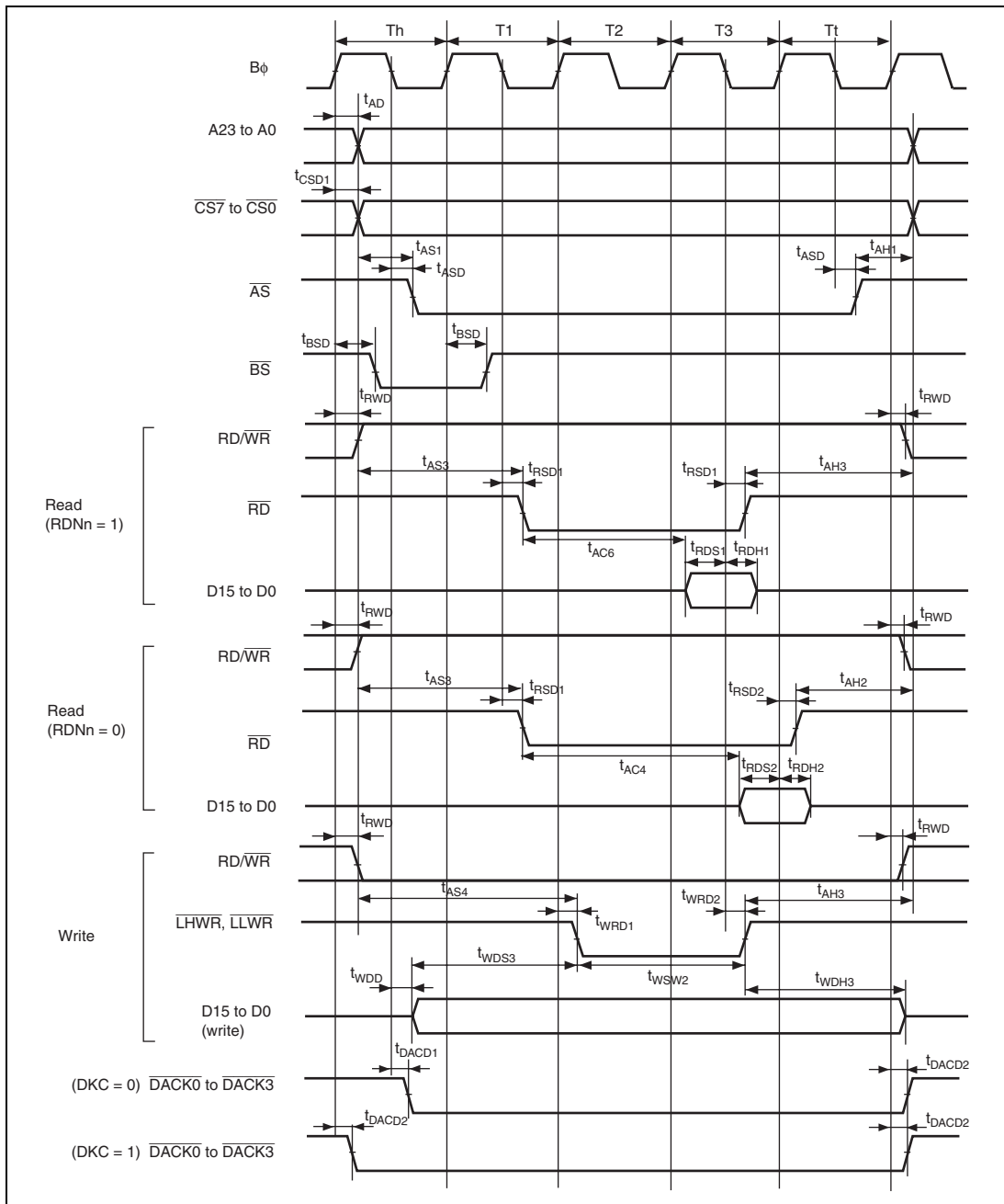
Figure 27.12 Basic Bus Timing: Three-State Access (CS Assertion Period Extended)
