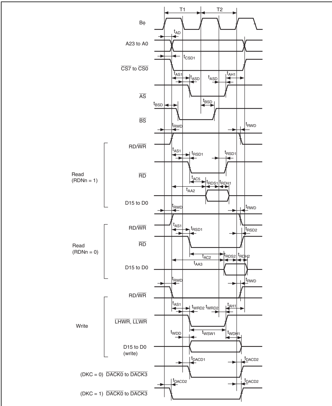
Figure 27.8 Basic Bus Timing: Two-State Access
