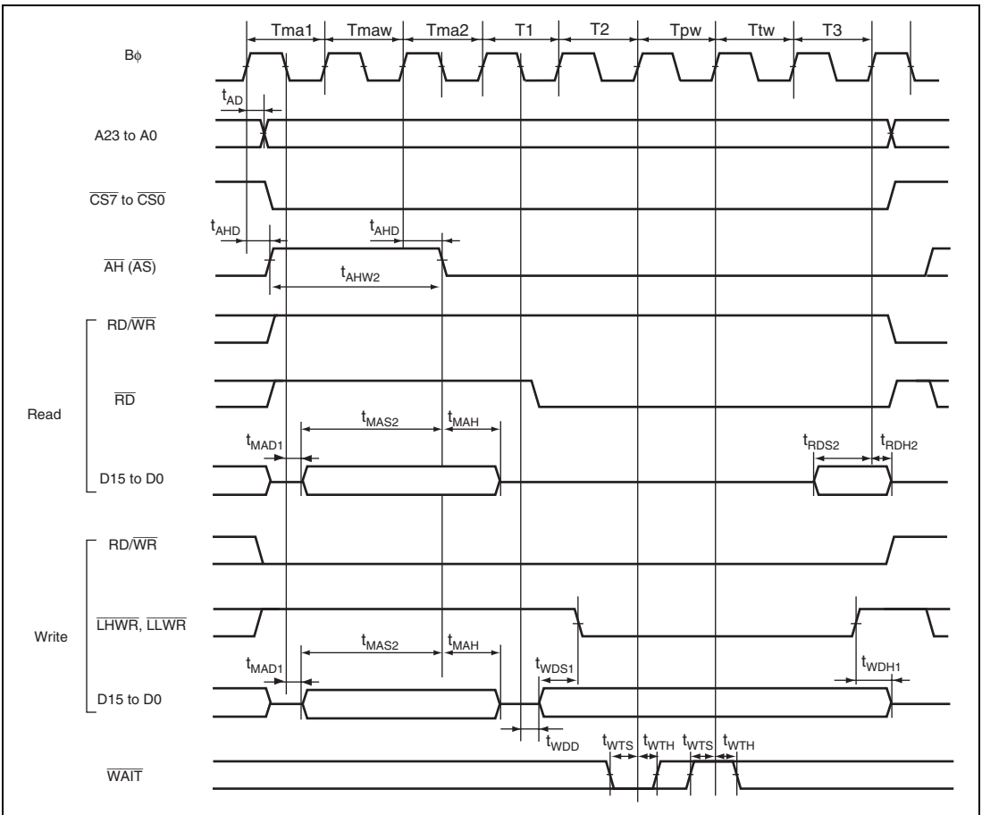
Figure 27.18 Address/Data Multiplexed Access Timing (Wait Control) (Address Cycle Program Wait × 1 + Data Cycle Program Wait × 1 + Data Cycle Pin Wait × 1)
