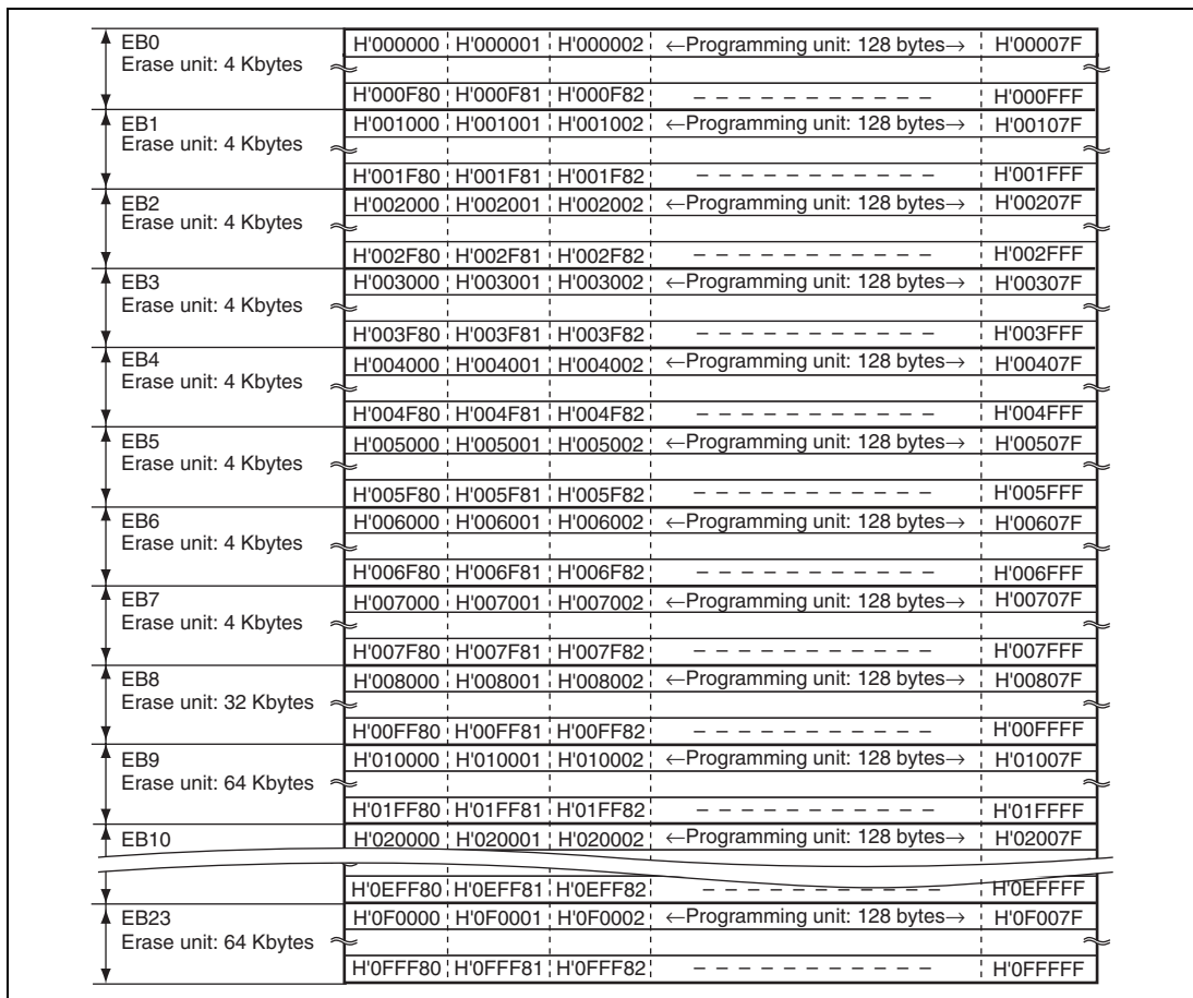
Figure 22.4 (3) User MAT Block Structure of H8SX/1638
