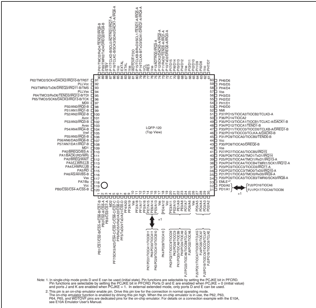
Figure 1.3 Pin Assignments
