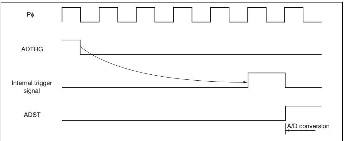
Figure 19.8 External Trigger Input Timing when Multiple Units Start Simultaneously (TRGS1, TRGS0, and EXTRGS = B'111)
