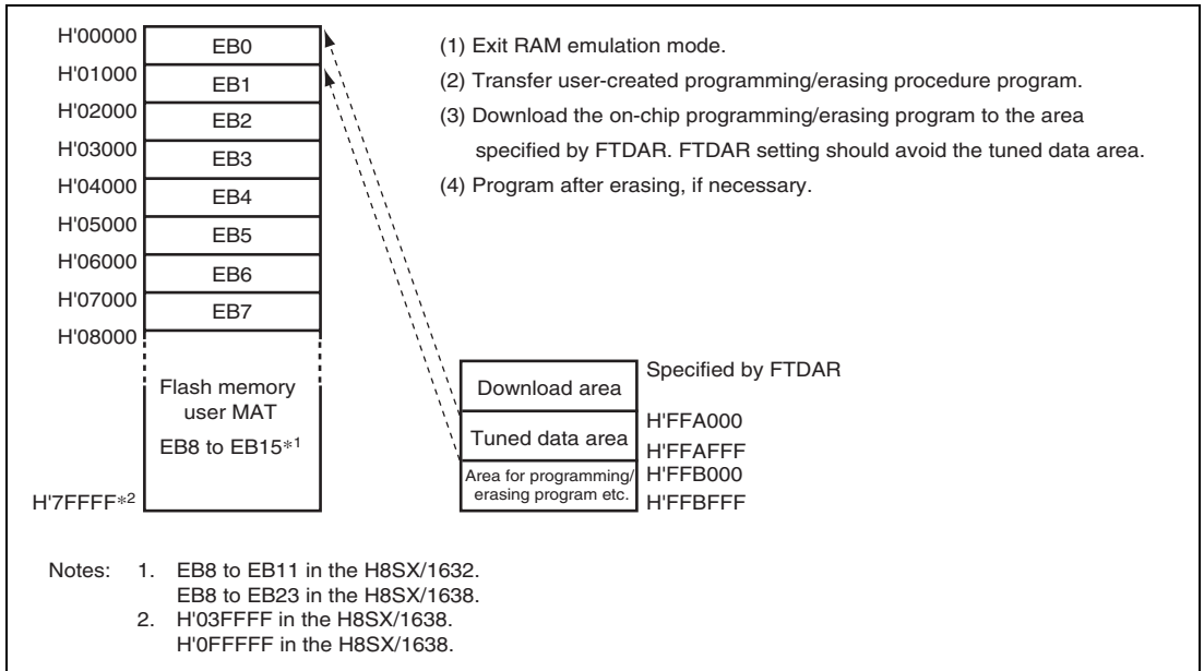
Figure 22.19 Programming Tuned Data (H8SX/1634)
