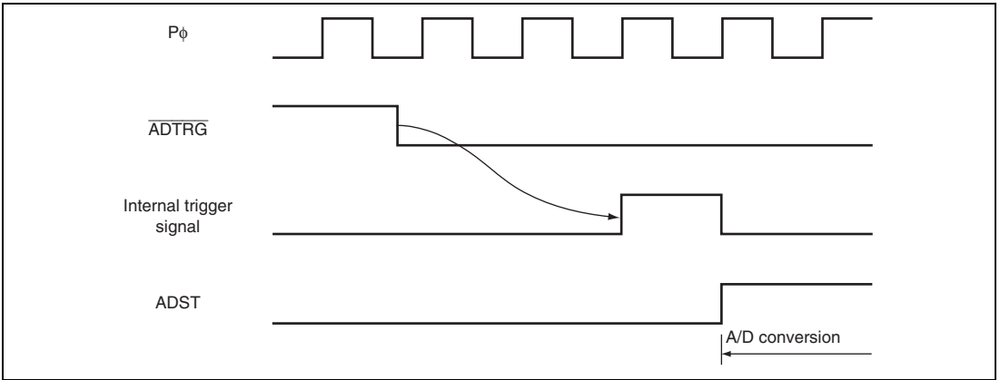
Figure 19.7 External Trigger Input Timing (TRGS1, TRGS0, and EXTRGS ≠ B'111)
