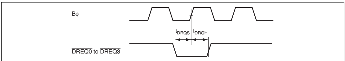
Figure 27.21 DMAC ( \overline{\text{DREQ}} ) Input Timing
