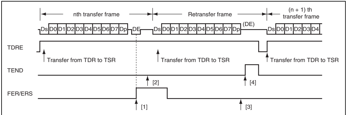
Figure 17.29 Data Re-Transfer Operation in SCI Transmission Mode
