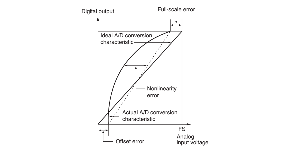
Figure 19.10 A/D Conversion Accuracy Definitions
