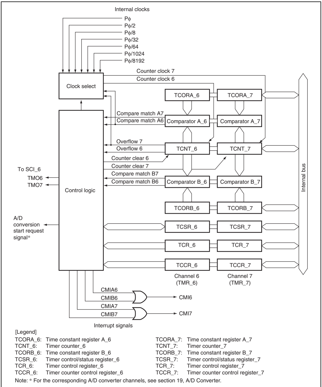
Figure 15.4 Block Diagram of 8-Bit Timer Module (Unit 3)
