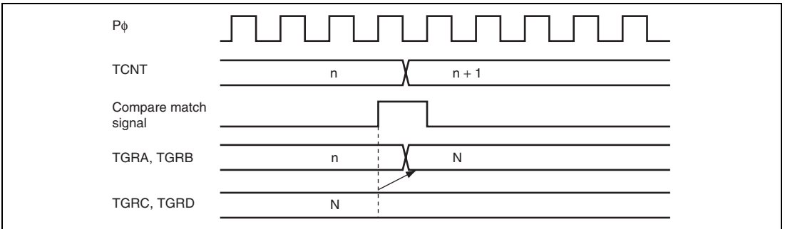
Figure 13.37 Buffer Operation Timing (Compare Match)
