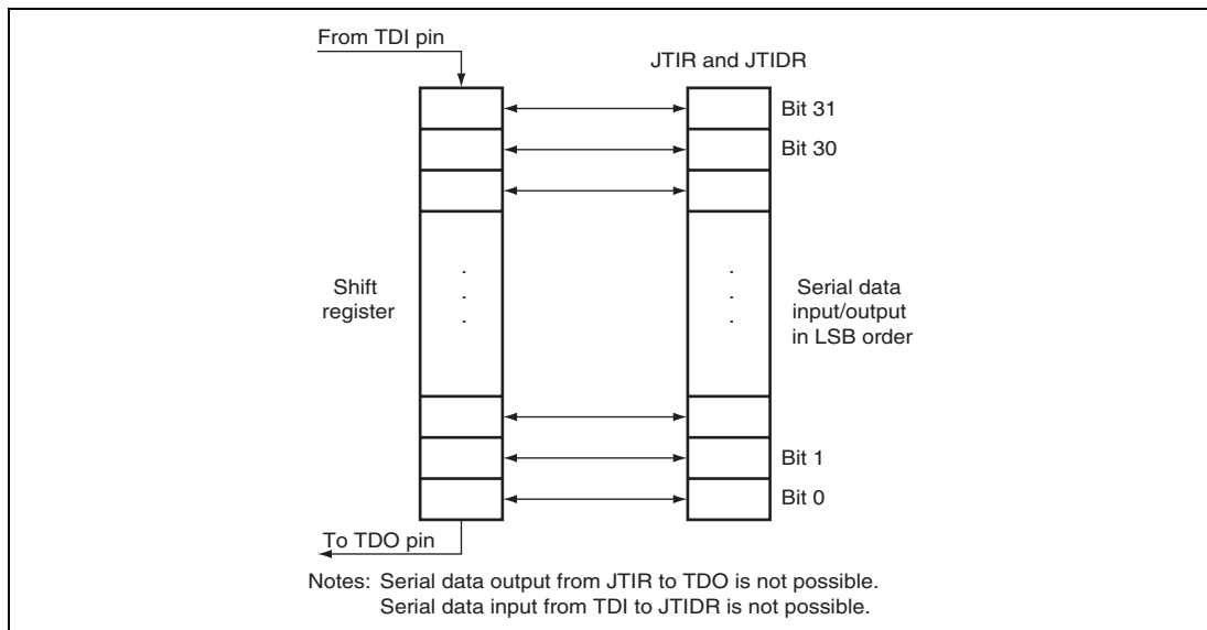
Figure 23.3 Serial Data Input/Output
