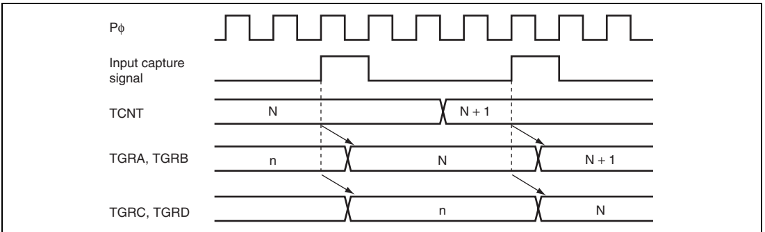
Figure 13.38 Buffer Operation Timing (Input Capture)
