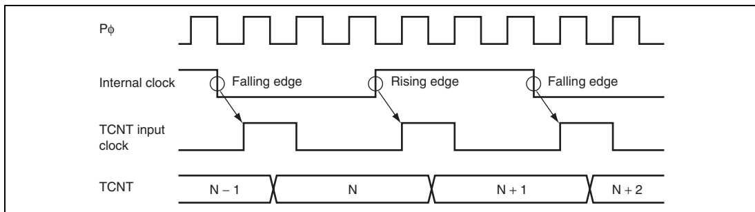
Figure 13.31 Count Timing in Internal Clock Operation
