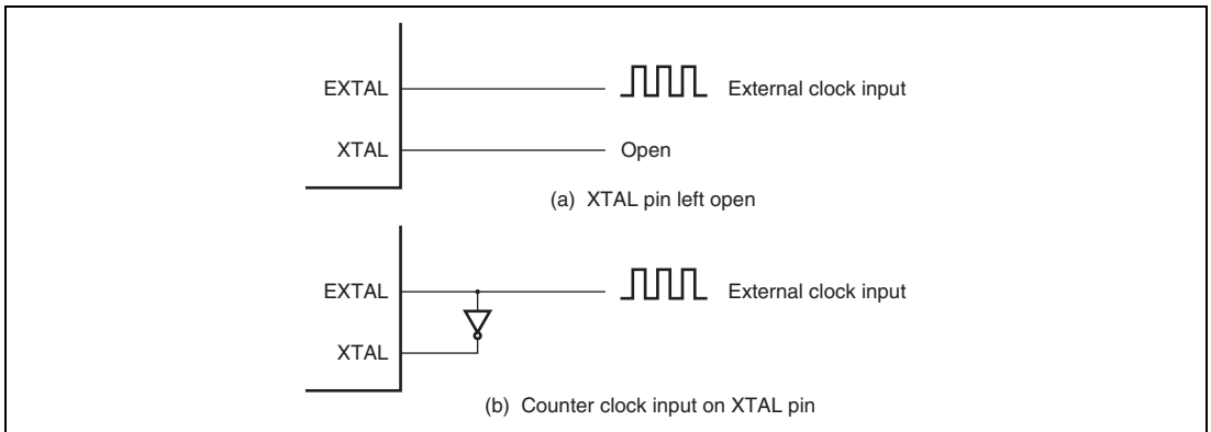
Figure 24.4 External Clock Input (Examples)
