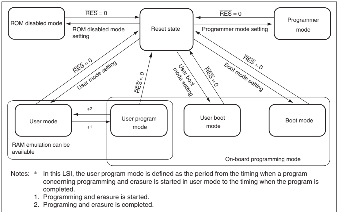
Figure 22.2 Mode Transition of Flash Memory
