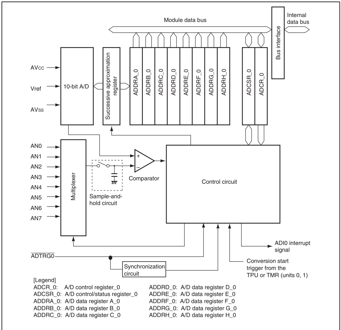
Figure 19.1 Block Diagram of A/D Converter Unit 0 (AD_0)
