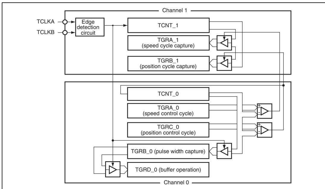
Figure 13.30 Phase Counting Mode Application Example
