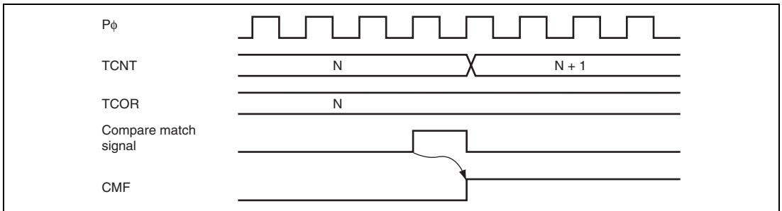
Figure 15.9 Timing of CMF Setting at Compare Match
