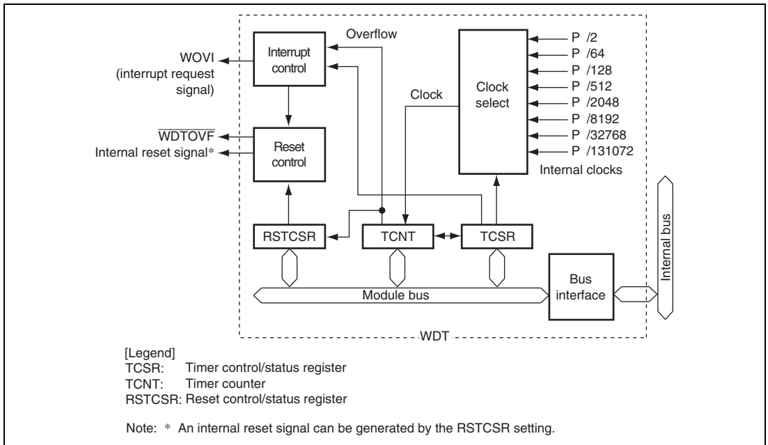
Figure 16.1 Block Diagram of WDT
