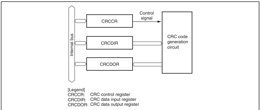
Figure 17.43 Block Diagram of CRC Operation Circuit
