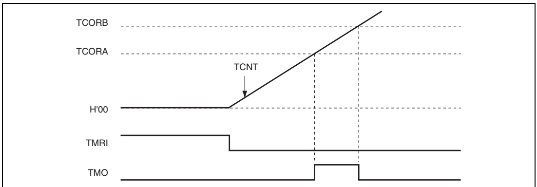
Figure 15.6 Example of Reset Input
