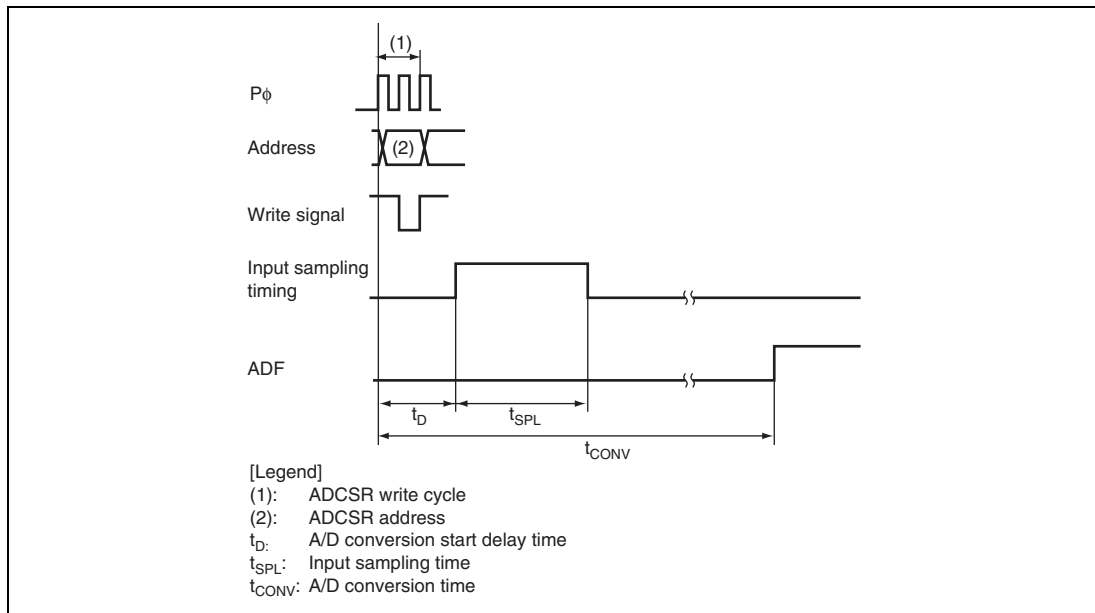
Figure 19.6 A/D Conversion Timing
