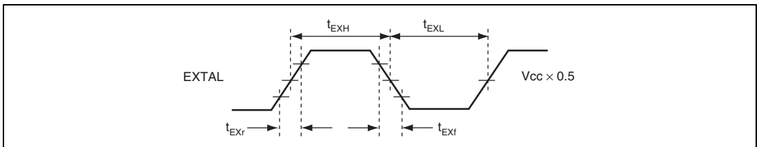
Figure 24.5 External Clock Input Timing
