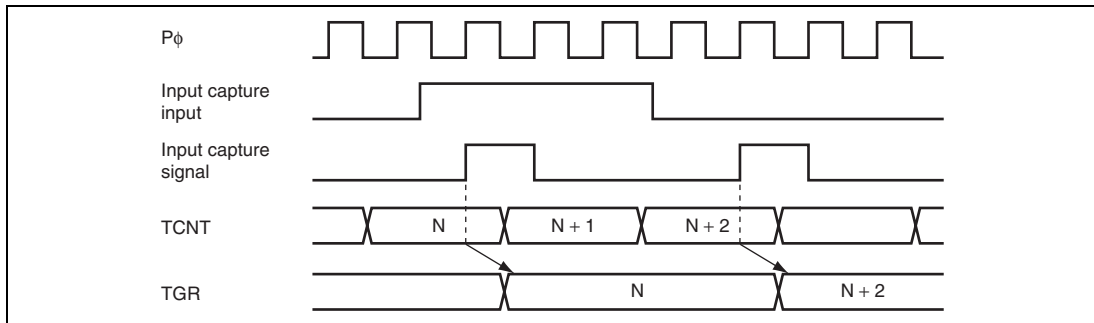
Figure 13.34 Input Capture Input Signal Timing
