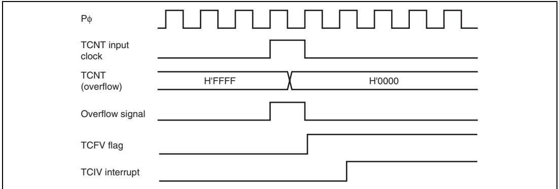
Figure 13.41 TCIV Interrupt Setting Timing
