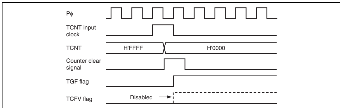
Figure 13.54 Conflict between Overflow and Counter Clearing
