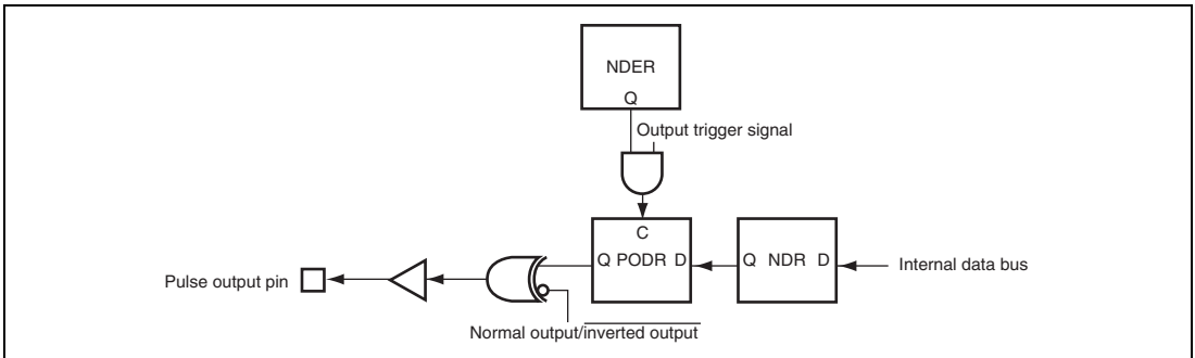
Figure 14.3 Schematic Diagram of PPG
