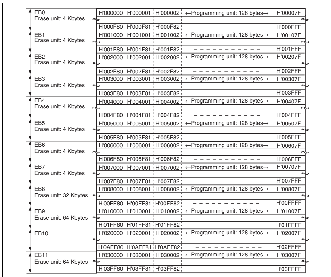
Figure 22.4 (1) User MAT Block Structure of H8SX/1632
