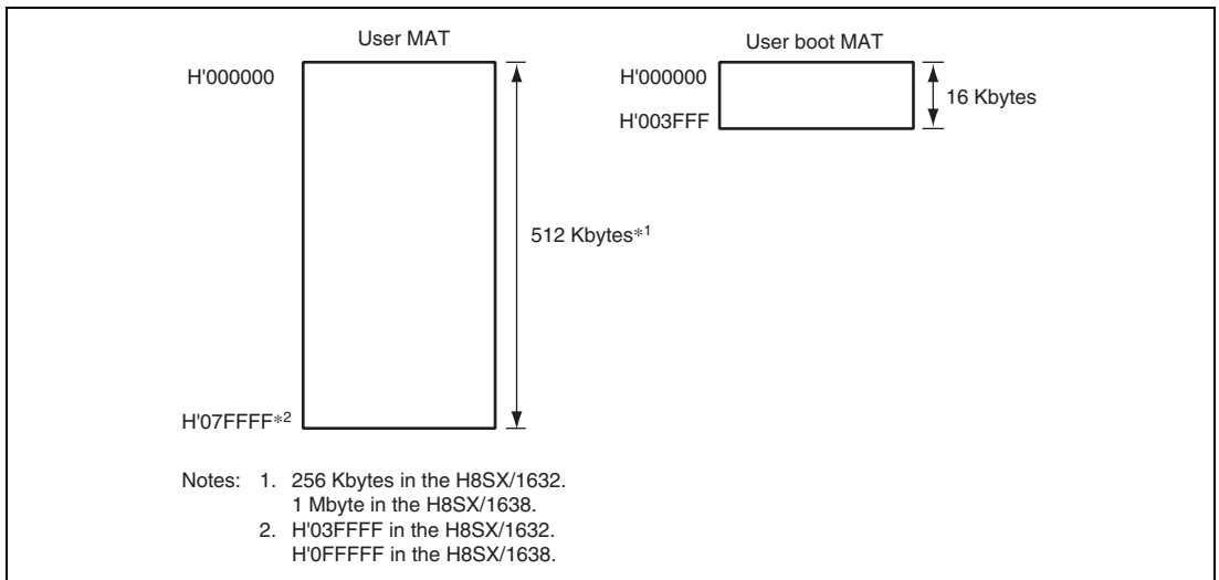
Figure 22.3 Memory MAT Configuration (H8SX/16xx_512K)
