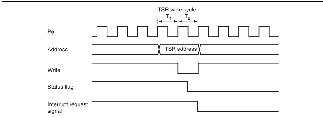
Figure 13.43 Timing for Status Flag Clearing by CPU
