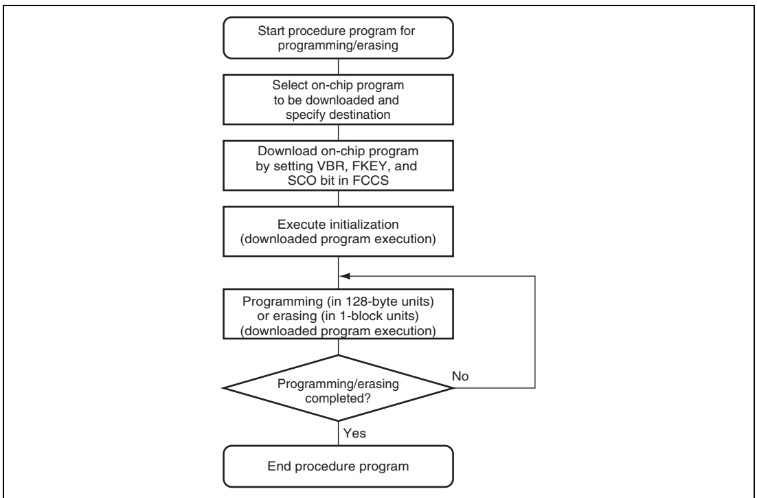
Figure 22.5 Procedure for Creating Procedure Program
