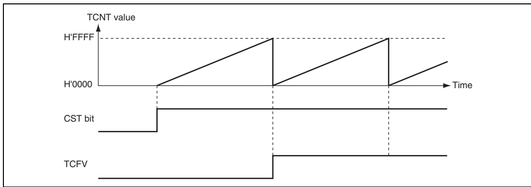
Figure 13.4 Free-Running Counter Operation
