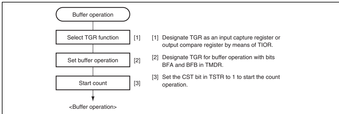
Figure 13.15 Example of Buffer Operation Setting Procedure
