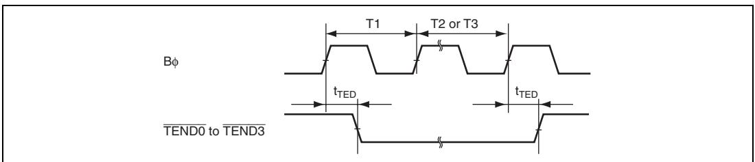
Figure 27.22 DMAC ( \overline{\text{TEND}} ) Output Timing
