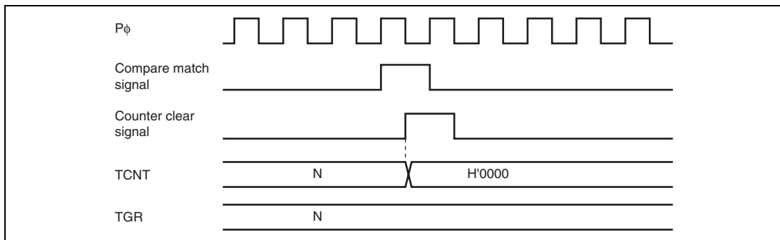
Figure 13.35 Counter Clear Timing (Compare Match)
