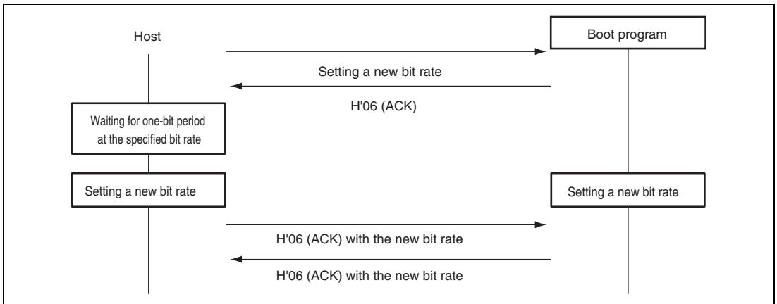
Figure 22.24 New Bit-Rate Selection Sequence
