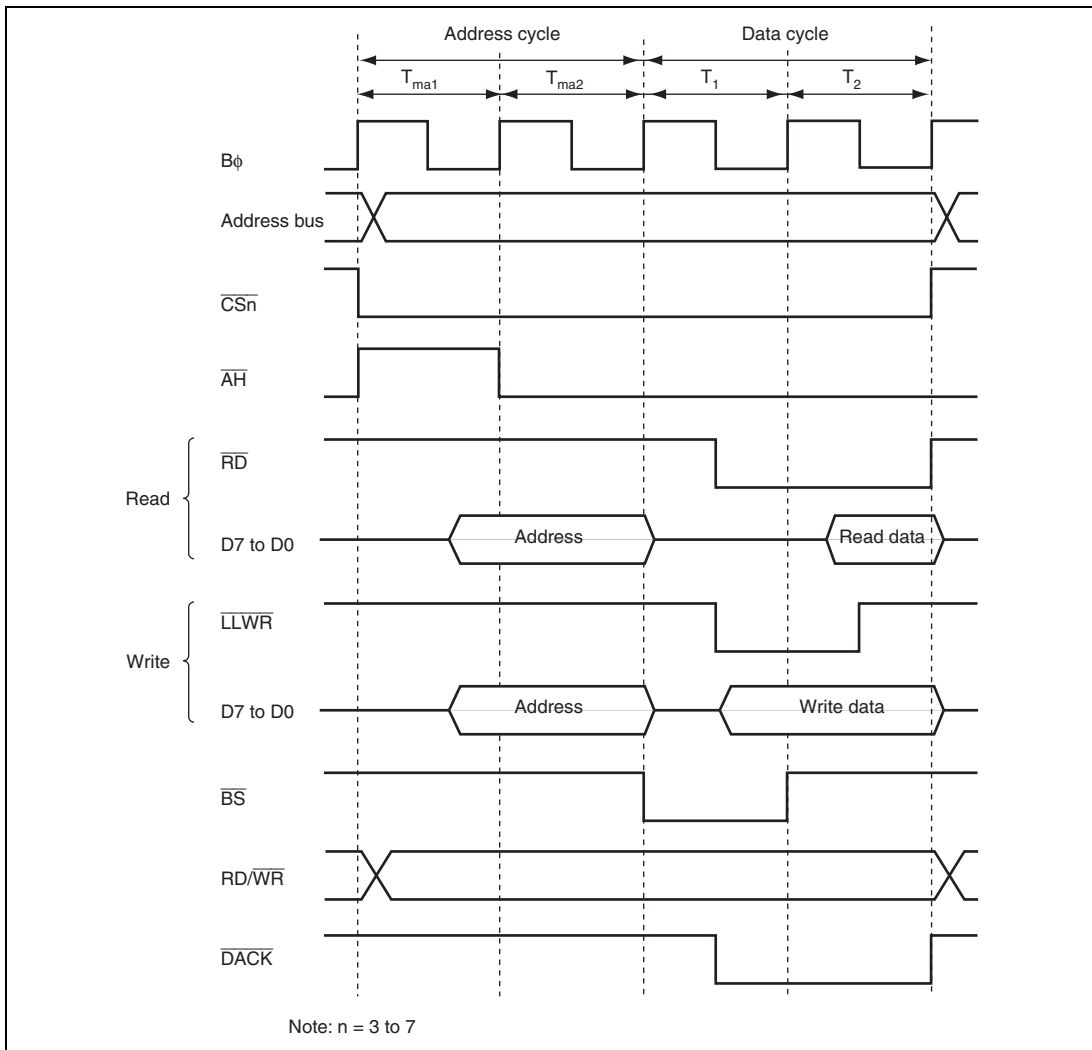
Figure 9.30 8-Bit Access Space Access Timing (ABWH n = 1, ABWL n = 1)
