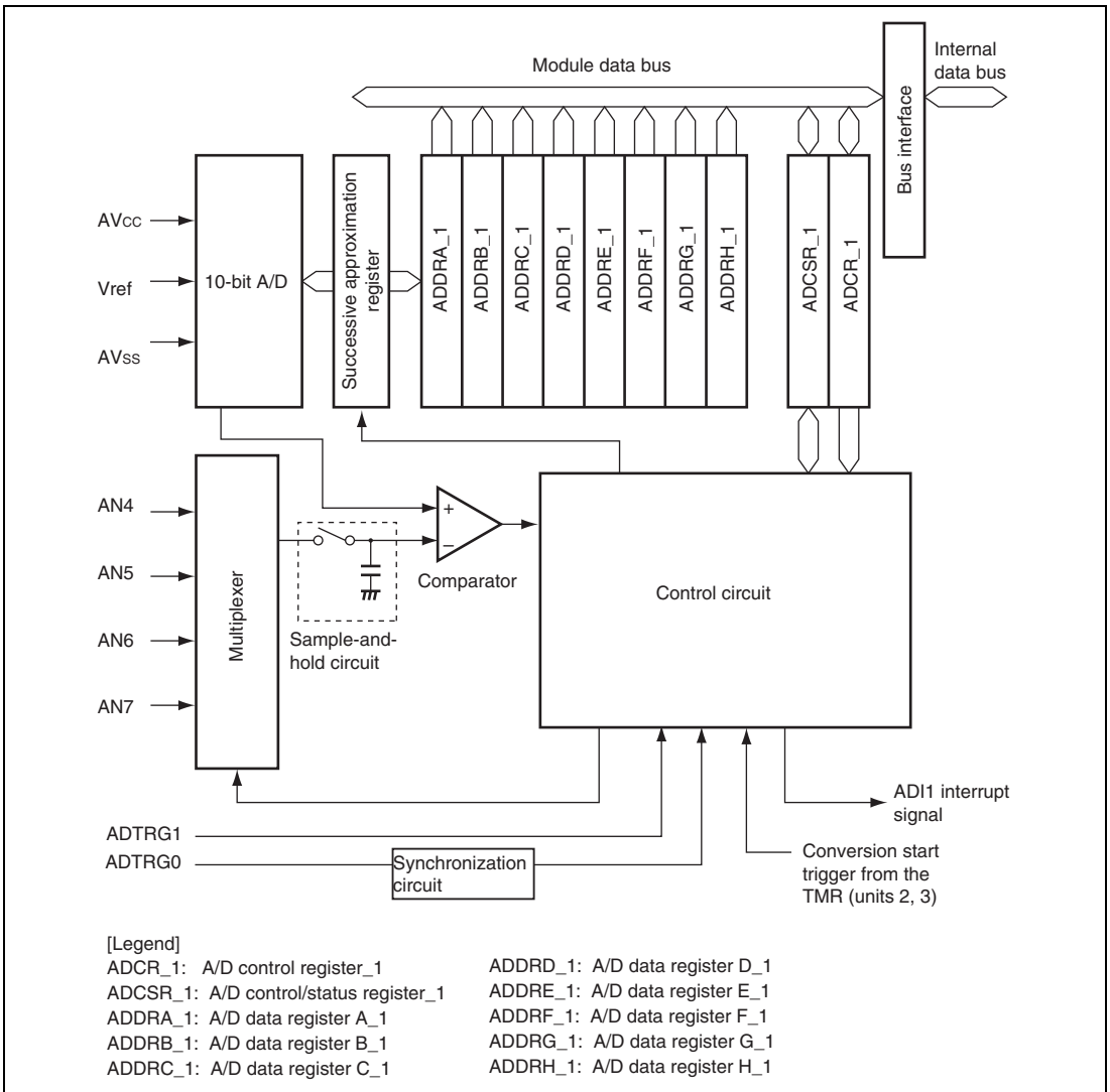
Figure 19.2 Block Diagram of A/D Converter Unit 1 (AD_1)
