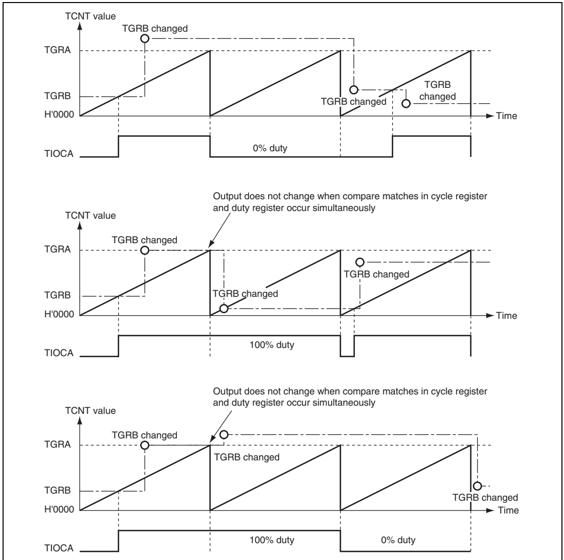
Figure 13.24 Example of PWM Mode Operation (3)
