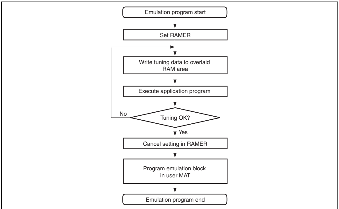
Figure 22.17 RAM Emulation Flow
