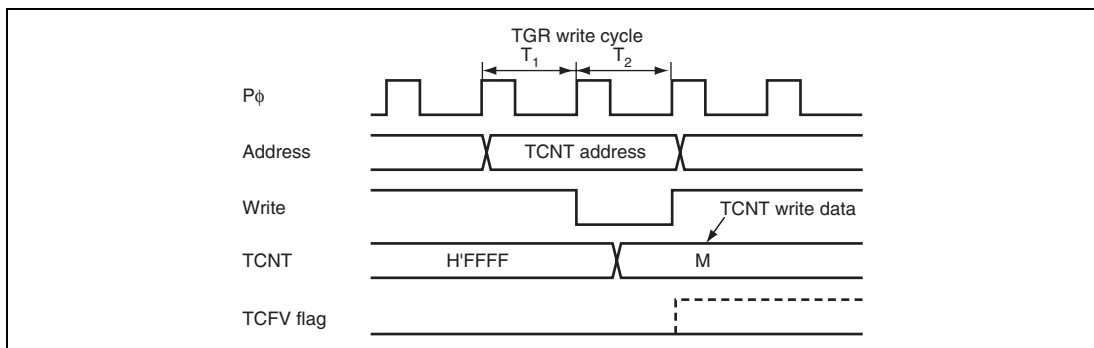
Figure 13.55 Conflict between TCNT Write and Overflow
