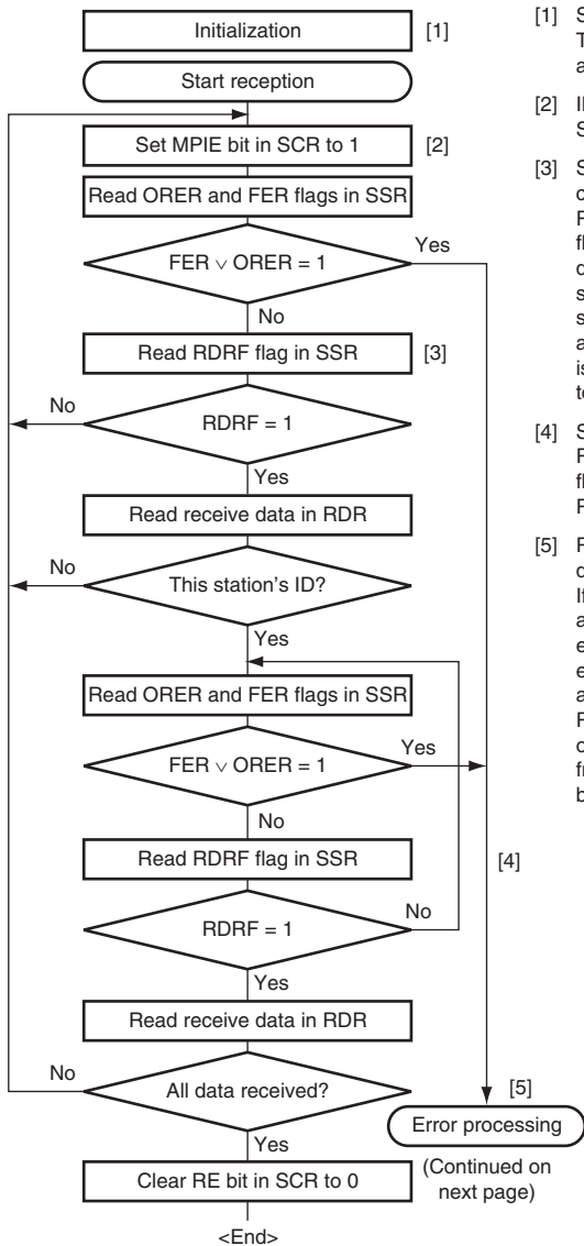
Figure 17.16 Sample Multiprocessor Serial Reception Flowchart (1)
