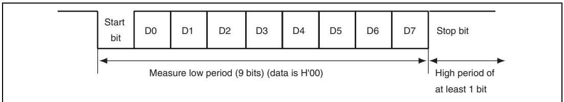
Figure 22.7 Automatic-Bit-Rate Adjustment Operation
