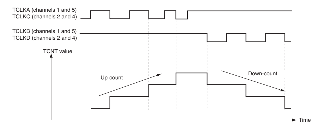
Figure 13.28 Example of Phase Counting Mode 3 Operation
