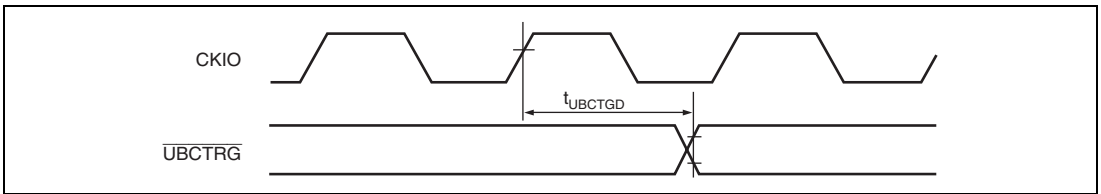
Figure 35.45 UBC Trigger Timing
