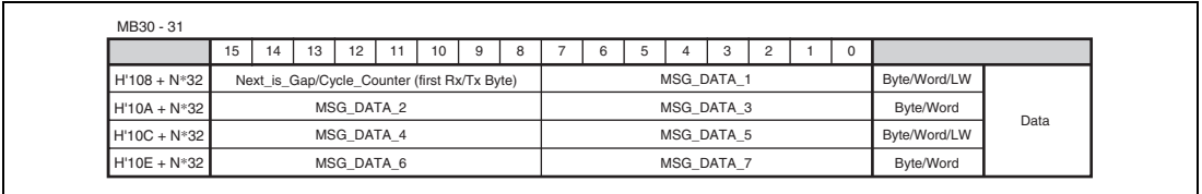
Figure 19.5 Message Data Field
