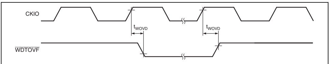
Figure 35.50 WDT Timing
