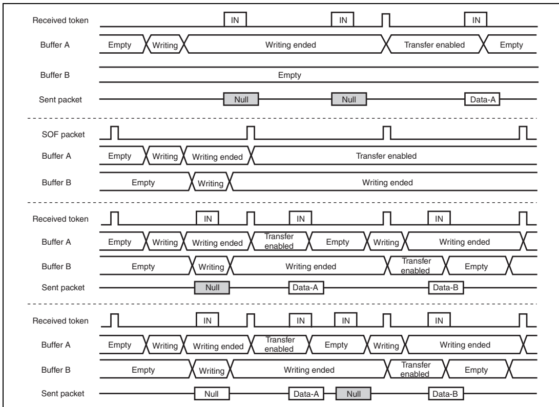
Figure 25.17 Example of Data Setup Function Operation
