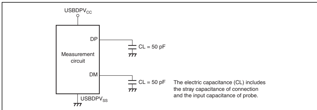
Figure 35.75 Measurement Circuit (Full-Speed)
