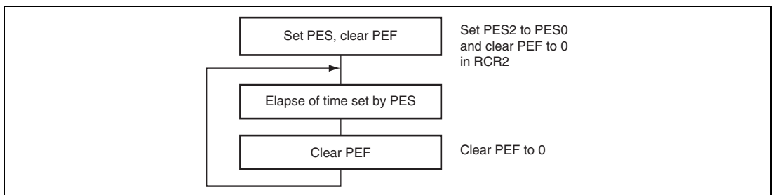
Figure 14.5 Using Periodic Interrupt Function
