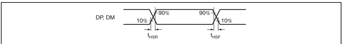
Figure 35.76 DP and DM Output Timing (High-Speed)
