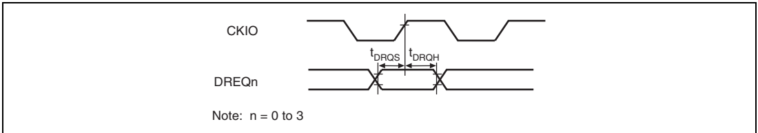
Figure 35.46 DREQ Input Timing
