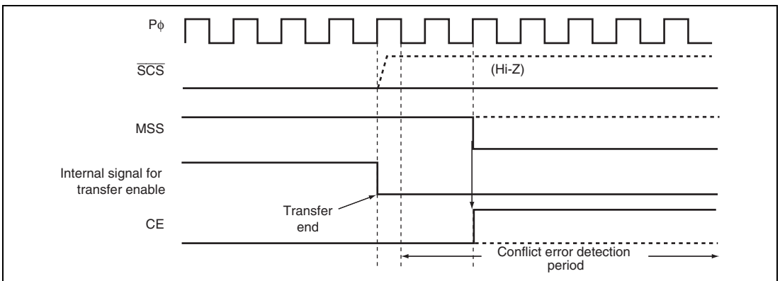
Figure 16.11 Conflict Error Detection Timing (After Transfer End)
