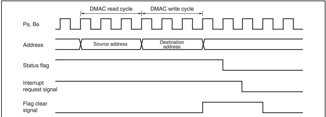
Figure 11.97 Timing for Status Flag Clearing by DMAC Activation
