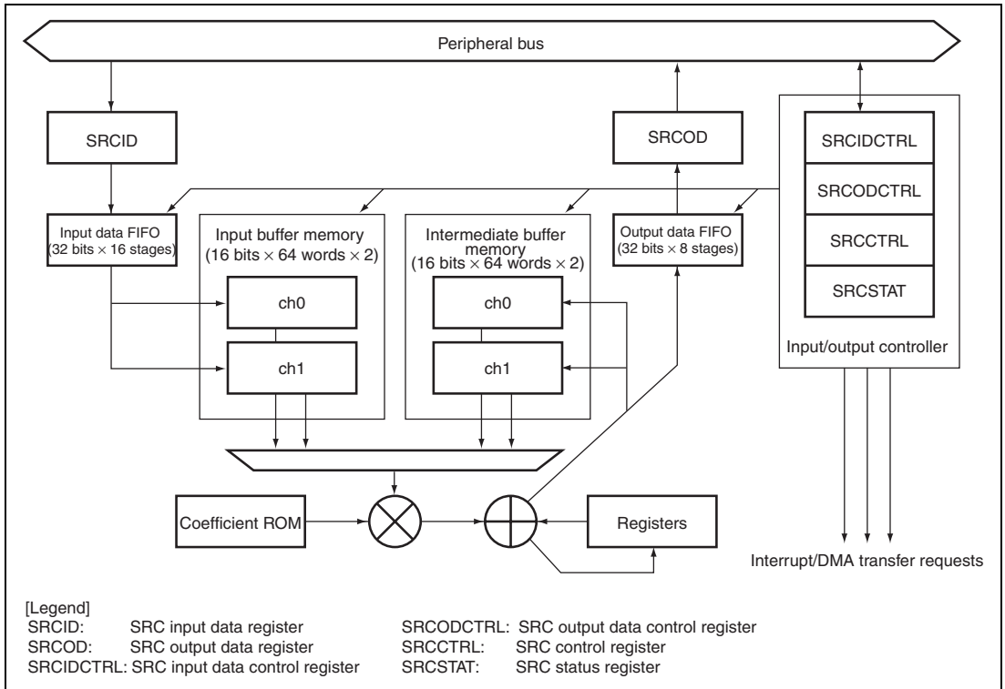
Figure 27.1 Block Diagram of SRC
