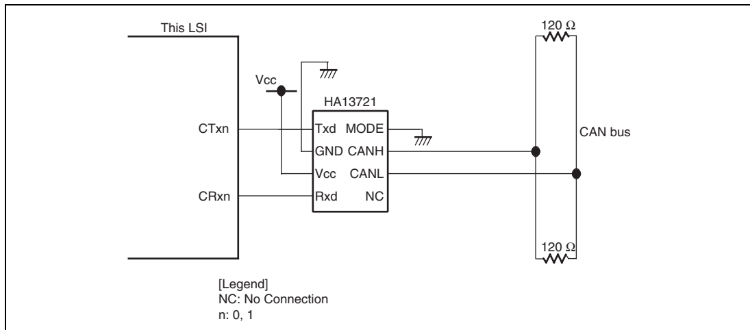
Figure 19.27 High-Speed CAN Interface Using HA13721
