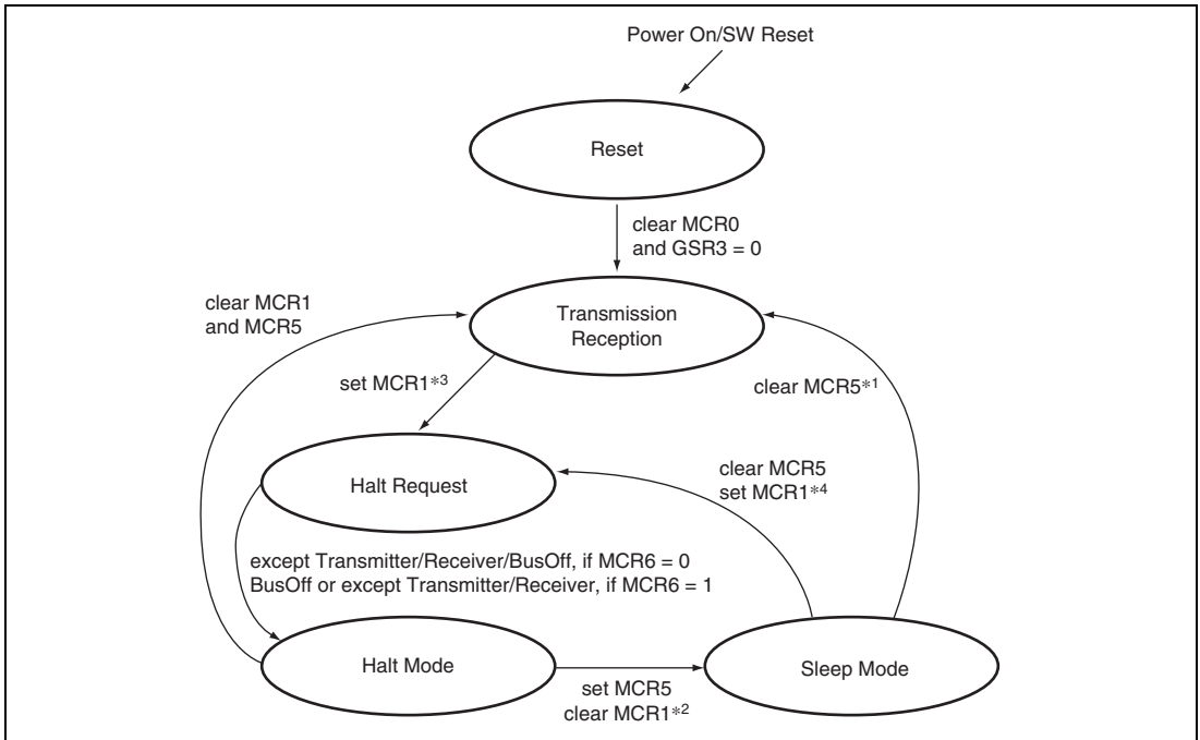
Figure 19.15 Halt Mode/Sleep Mode
