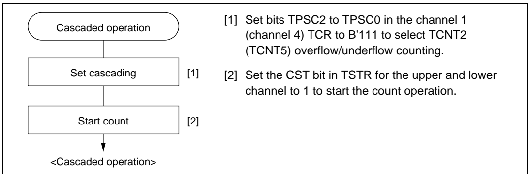
Figure 9.21 Cascaded Operation Setting Procedure
