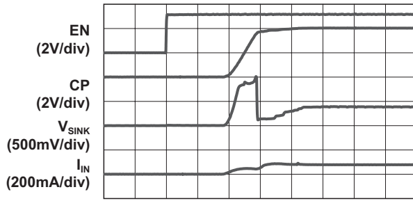
Turn-On to 1X Mode ( V_{IN} = 4.2V ; 20mA Load)
