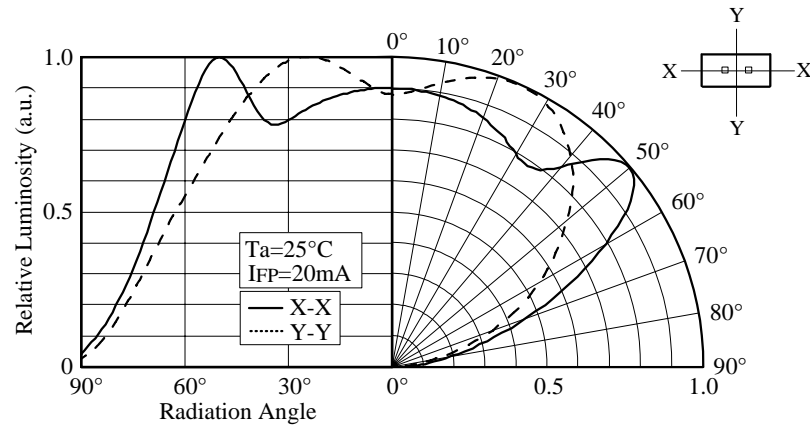
■ Directivity
