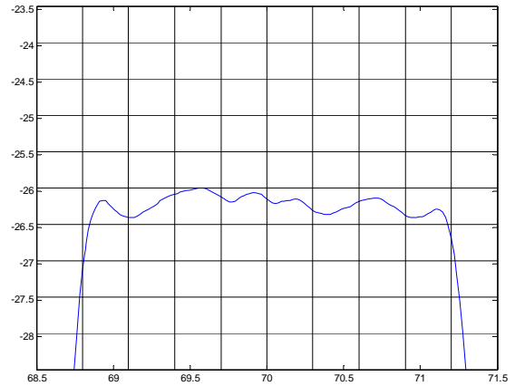
Phase Linearity( f_0 \pm 1.1\text{MHz} )
