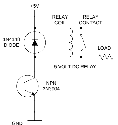
[EXAMPLE] NPN RELAY DRIVE CIRCUIT FOR RECEIVER
