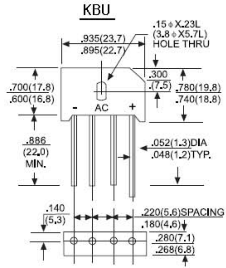
Dimensions in inches and (millimeters)
