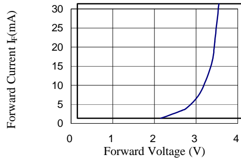
FIG.2 FORWARD CURRENT I F (mA) VS. FORWARD VOLTAGE
