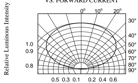
FIG.6 RADIATION DIAGRAM
