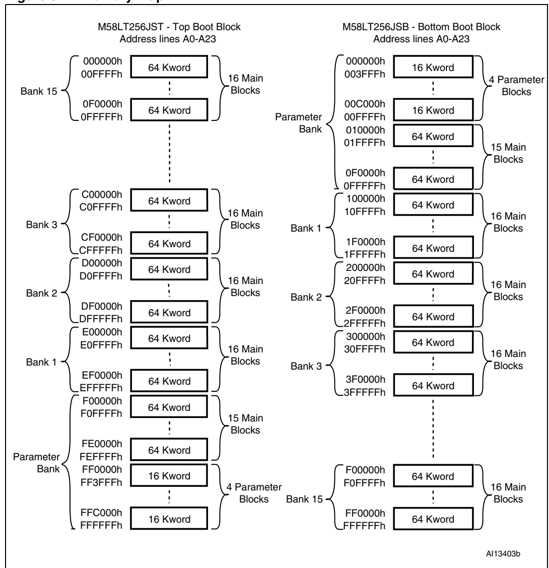
Figure 3. Memory map
